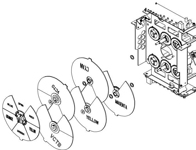
Figure 4-3 x.SpotXtreme color wheel assembly
