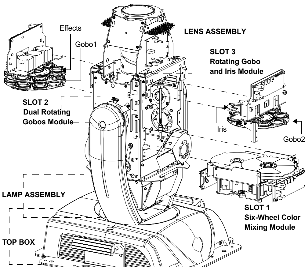
Figure 1-1 x.SpotXtreme Fixture Components
