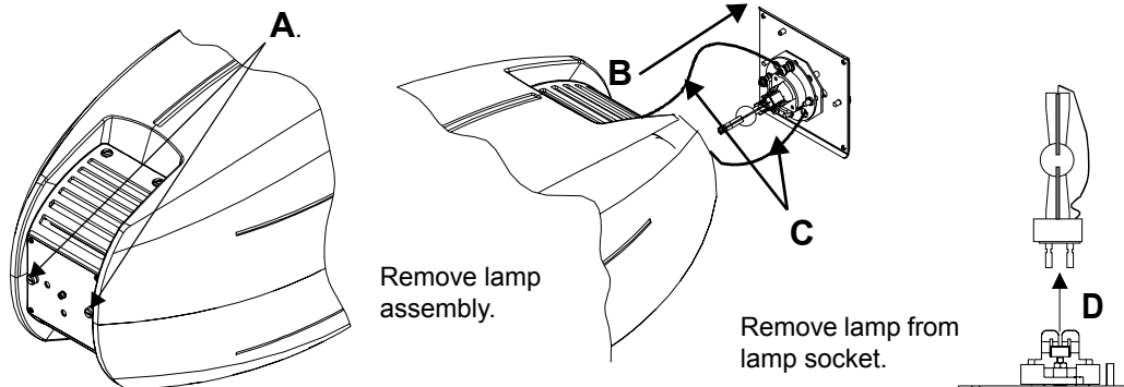
Figure 5-3 Replacing the lamp
