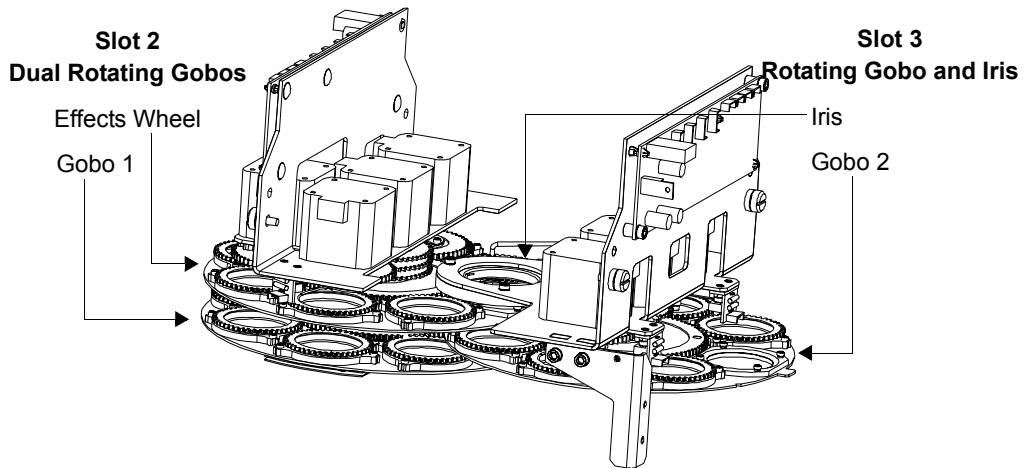
Figure 1-2 Module Interleaving in Standard x.Spot®Xtreme fixture
