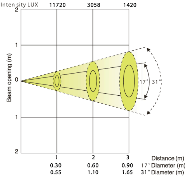
Beam angle 17° Field angle 31° - All LEDs (25° Lens)
