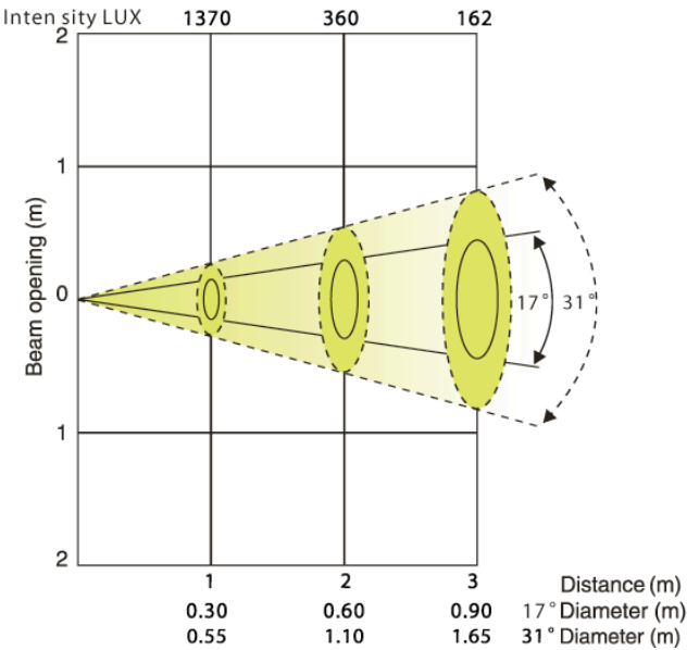
Beam angle 17° Field angle 31° - Blue LEDs (25° Lens)
