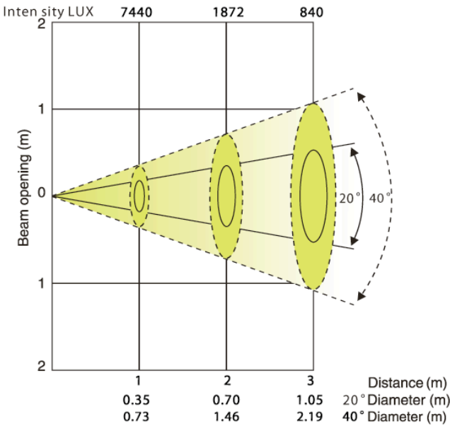
Beam angle 20° Field angle 40° - Red LEDs (45° Lens)
