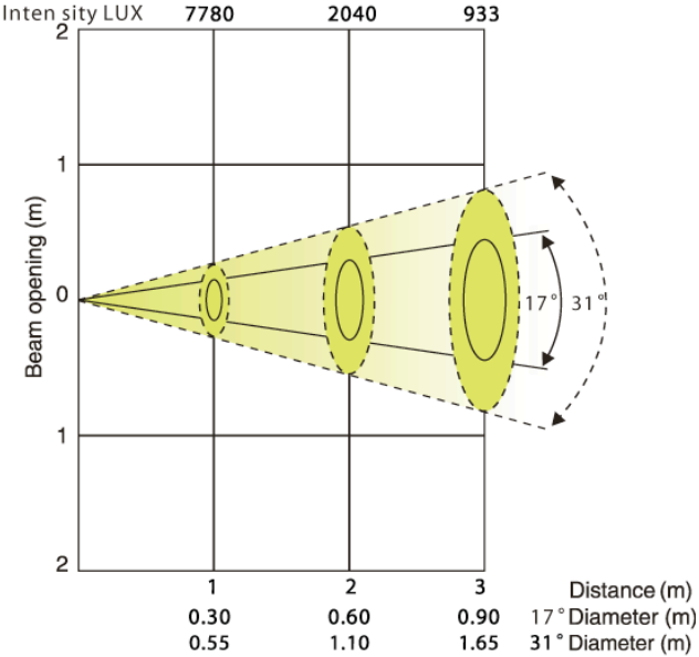
Beam angle 17° Field angle 31° - Green LEDs (25° Lens)
