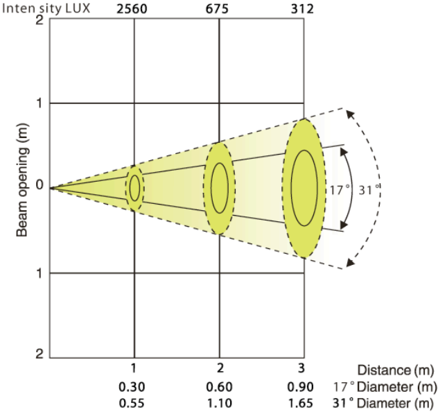
Beam angle 17° Field angle 31° - Red LEDs (25° Lens)
