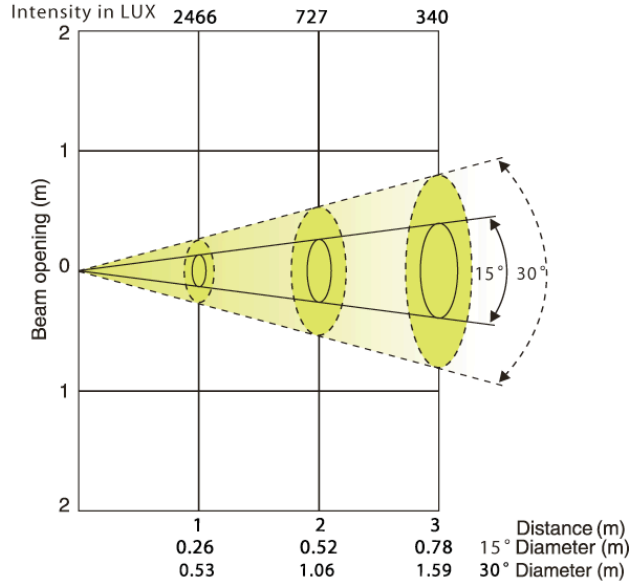
All Green LEDs - 15° Beam Angle/30° Field Angle
