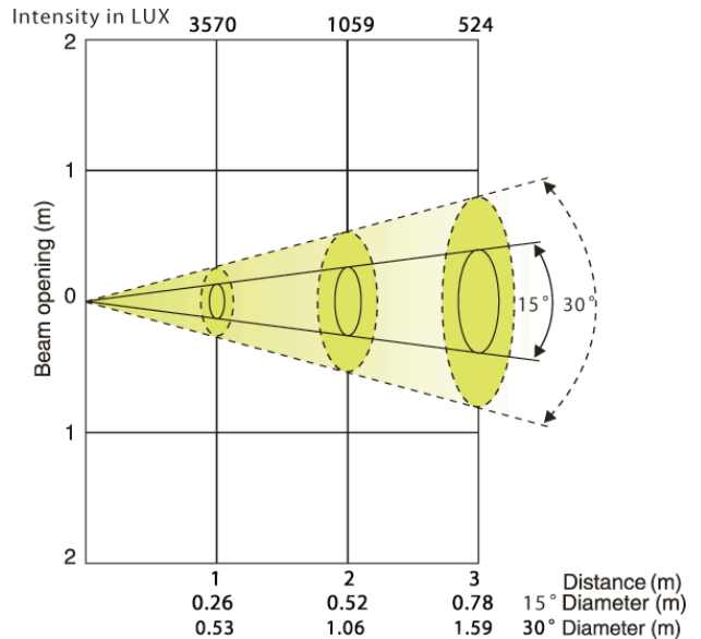
All LEDs - 15° Beam Angle/30° Field Angle
