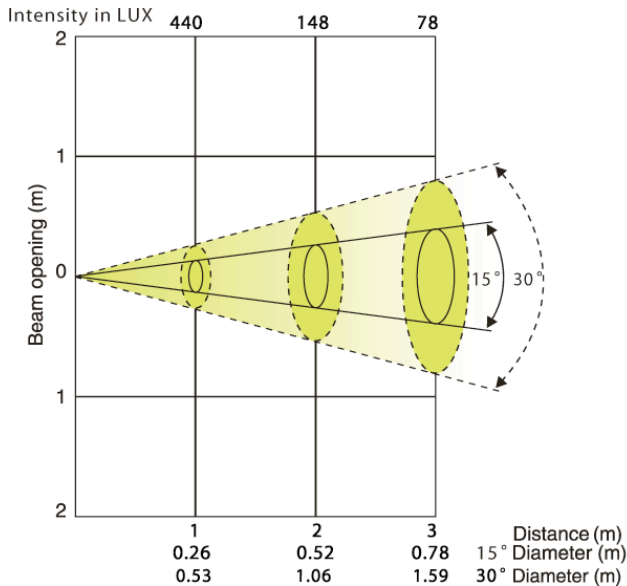
All BlueLEDs - 15° Beam Angle/30° Field Angle
