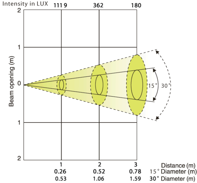
All Red LEDs - 15° Beam Angle/30° Field Angle
