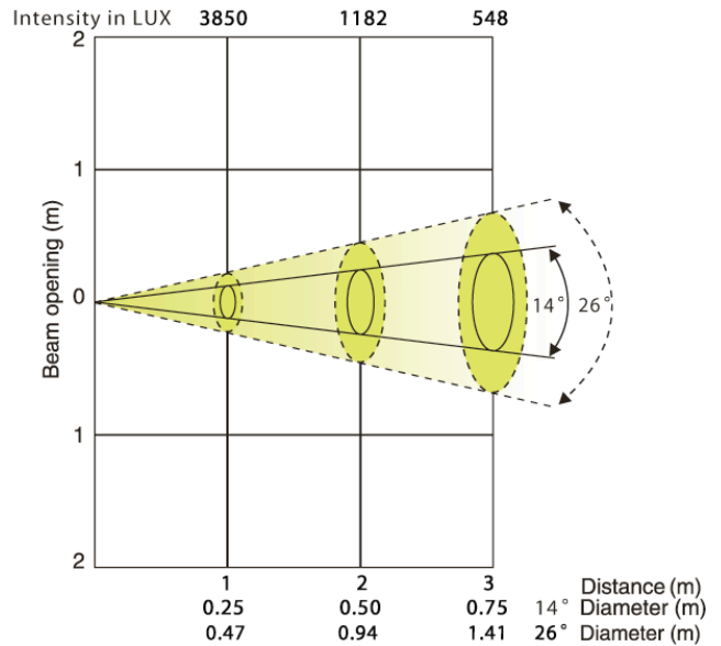
All LEDs - 14° Beam Angle/26° Field Angle
