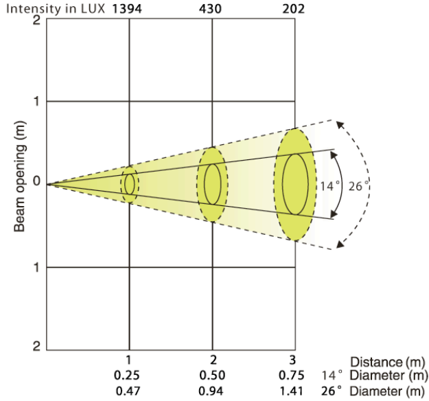
All Red LEDs - 14° Beam Angle/26° Field Angle
