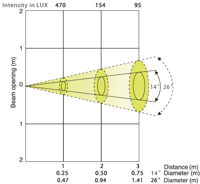
All BlueLEDs - 14° Beam Angle/26° Field Angle
