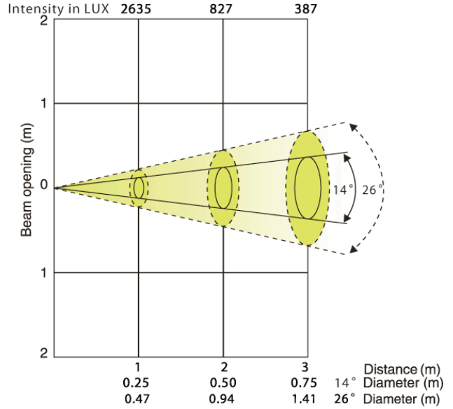
All Green LEDs - 14° Beam Angle/26° Field Angle
