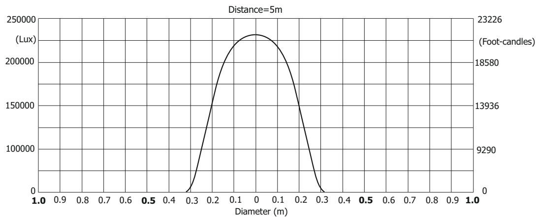
Illuminance distribution
