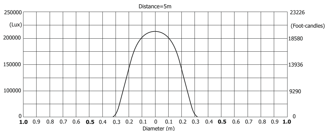
Illuminance distribution
