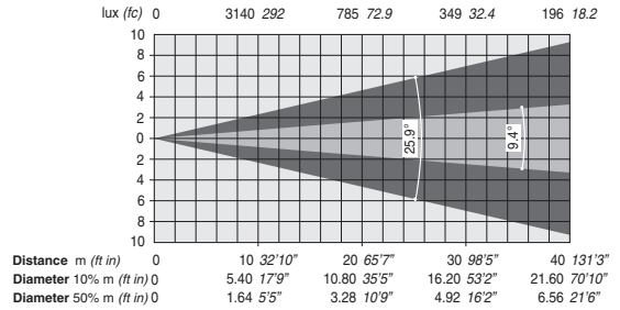
Maximum Zoom (25.9° 10% - 9.4° 50%)
