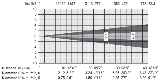
Minimum Zoom (12.1° 10% - 4.3° 50%)
