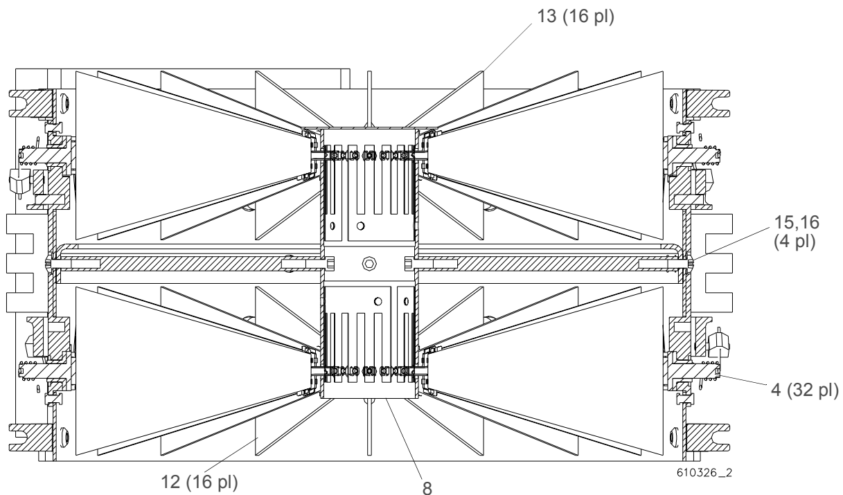
Figure 3-15: Blue/Magenta Bulkhead Assembly (cut-away view)
