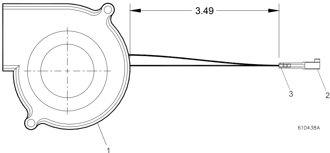
Figure 3-9: Color Motor/Lamp Fan Assembly
