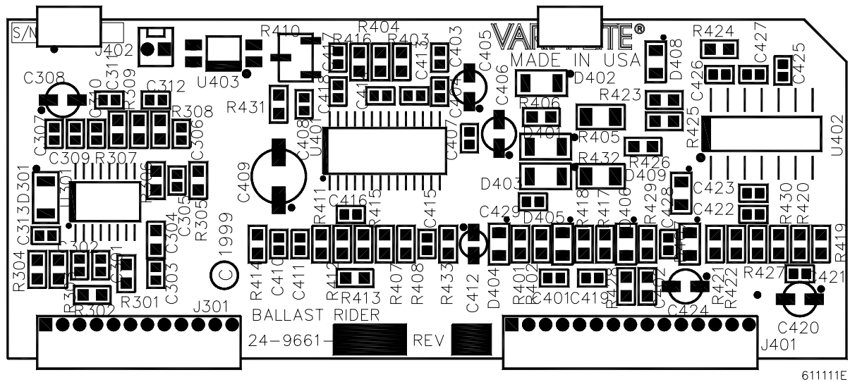
Figure 3-61: 1200W Ballast Rider PCB Assembly
