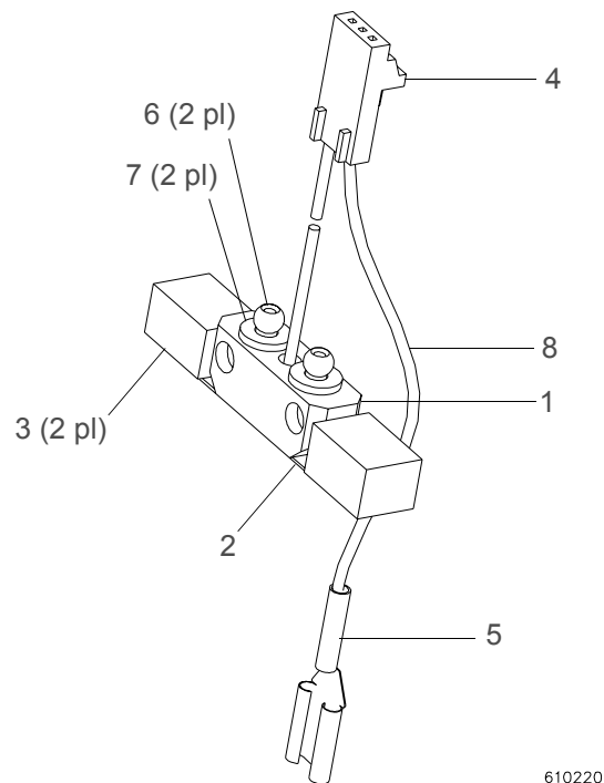
Figure 3-29: Bulb Disconnect Assembly
