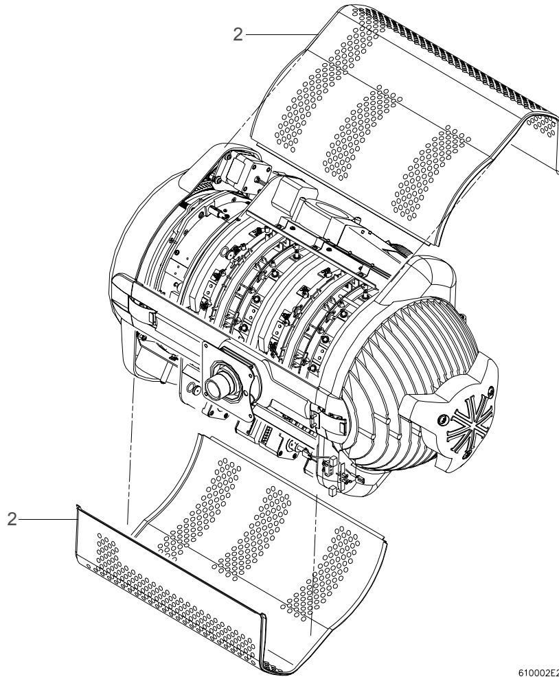
Figure 3-3: Head Covers
