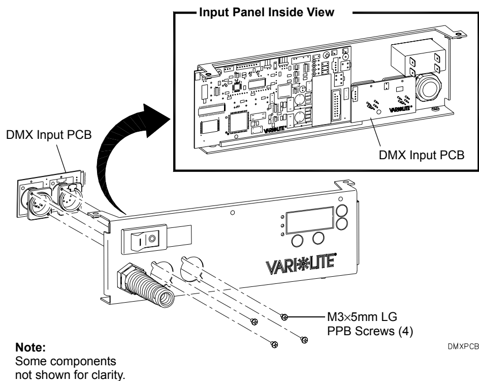
Figure 2-22: DMX Input PCB Assembly Replacement
