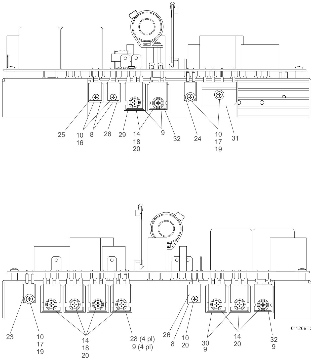
Figure 3-59: 1200W Arc Ballast Module Assembly (side views)
