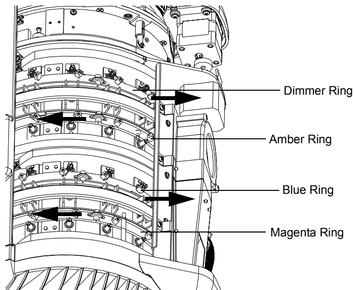
Figure 2-8: Closing Filters
