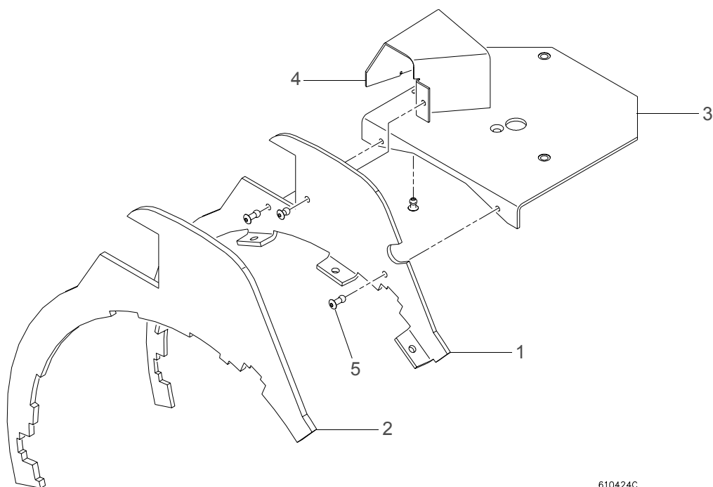
Figure 3-36: Beam Spreader Heat Shield Assembly
