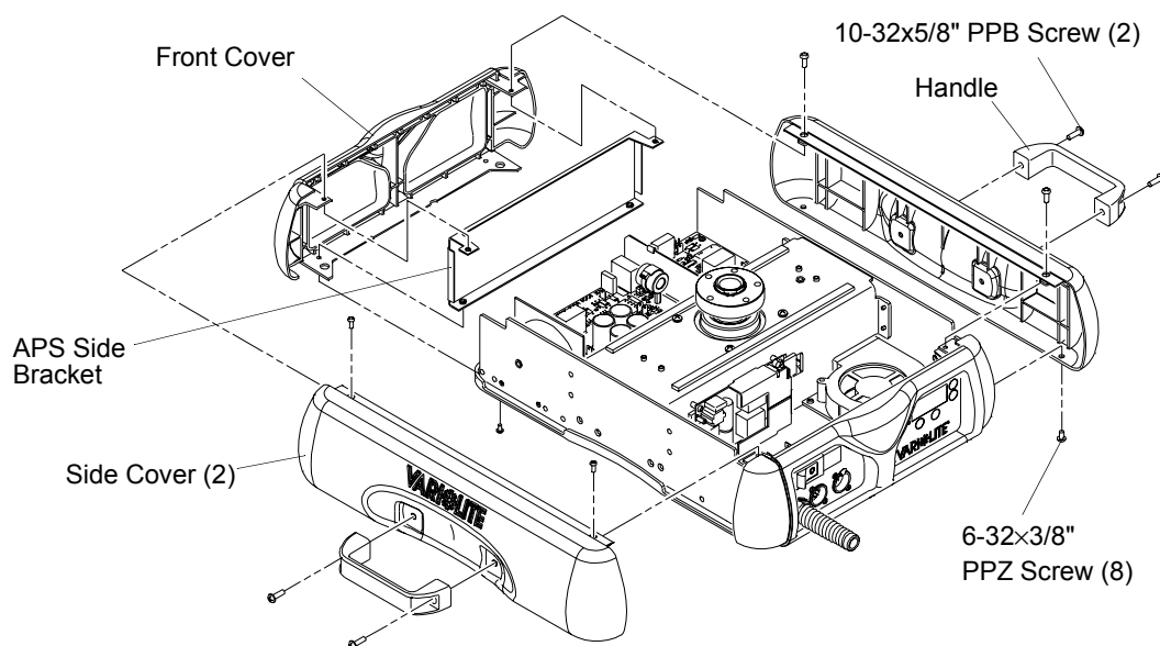
Figure 2-17: Accessing Ballast Module
