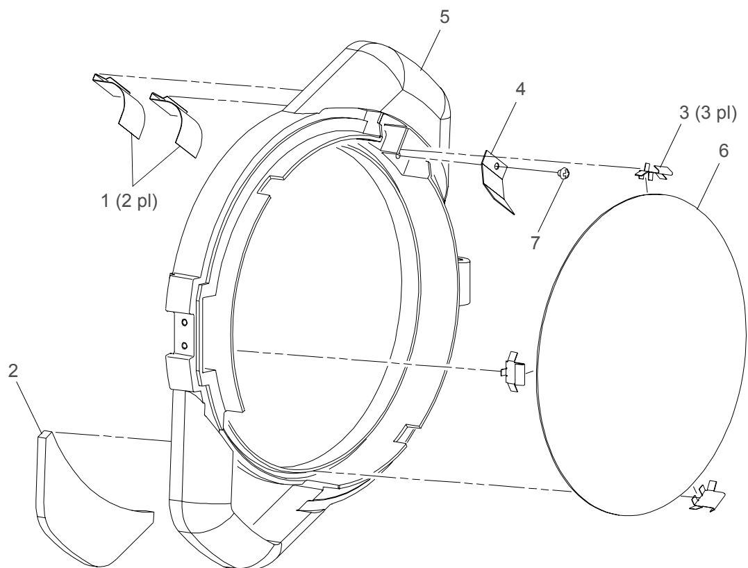
Figure 3-7: Cooling Bulkhead Assembly VL2413/VL2414/VL2415/VL2416
