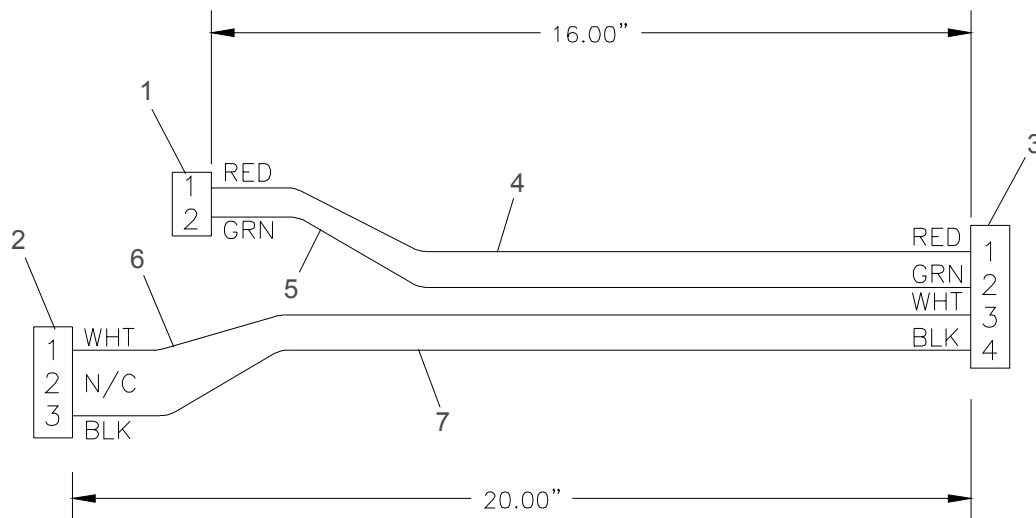
Figure 3-79: Lamp Supply OT/NOT On Cable Assembly
