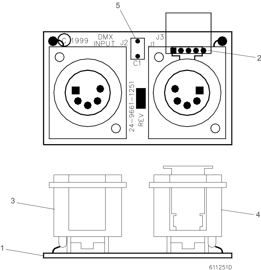
Figure 3-49: DMX Input PCB Assembly
