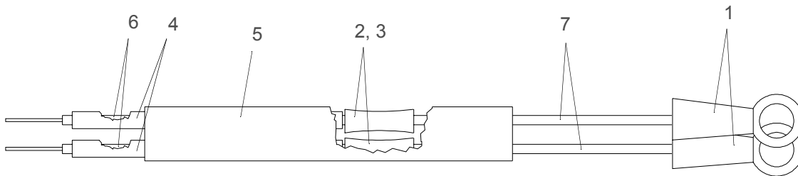
Figure 3-77: Bulb Socket to Ignitor Cable Assembly
