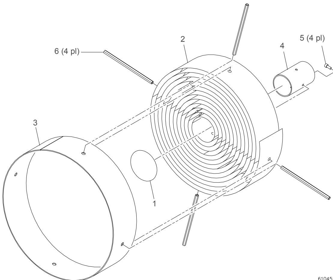
Figure 3-39: Light Baffle Center Assembly
