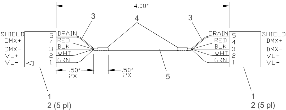
Figure 3-80: Data I/O Link Cable Assembly
