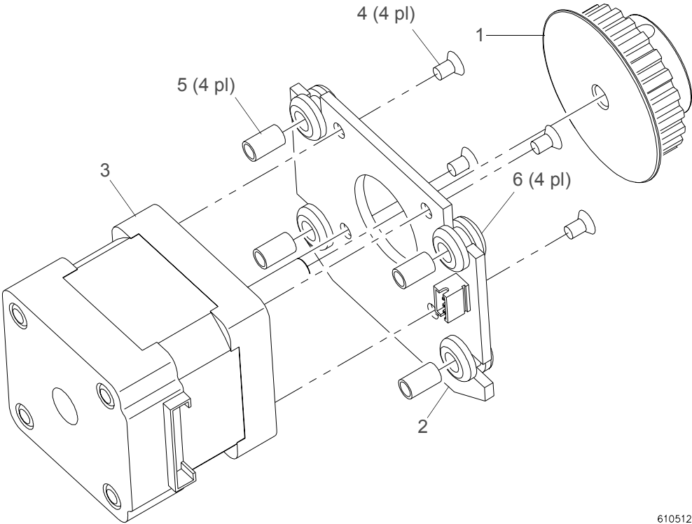
Figure 3-11: Drive Motor Assembly
