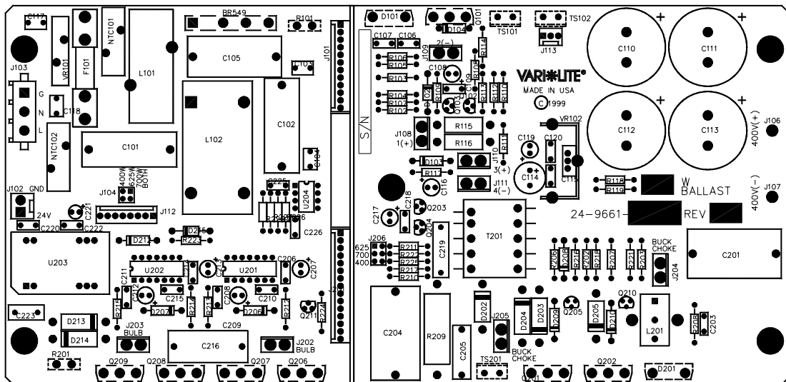
Figure 3-56: 400/625W Ballast Board PCB Assembly
