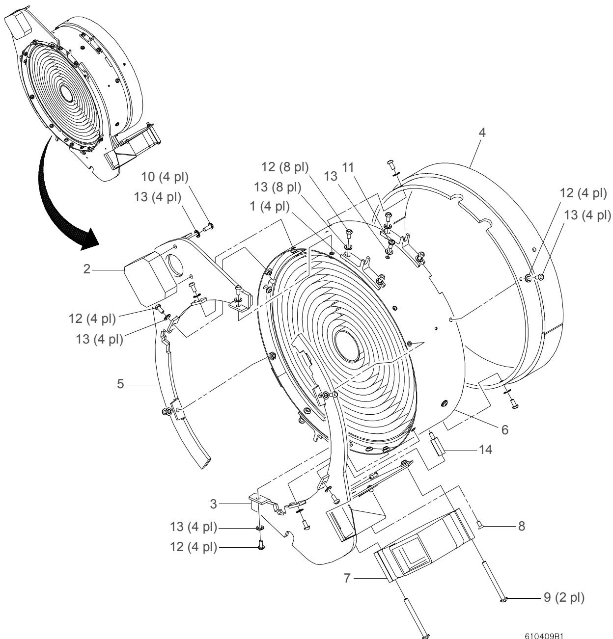
Figure 3-30: Light Baffle w/ Counter Weight Assembly
