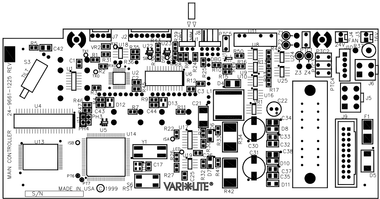
Figure 3-48: Main Controller 3-Phase PCB Assembly
