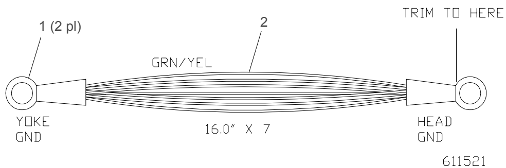
Figure 3-73: Yoke to Head Ground Cable Assembly
