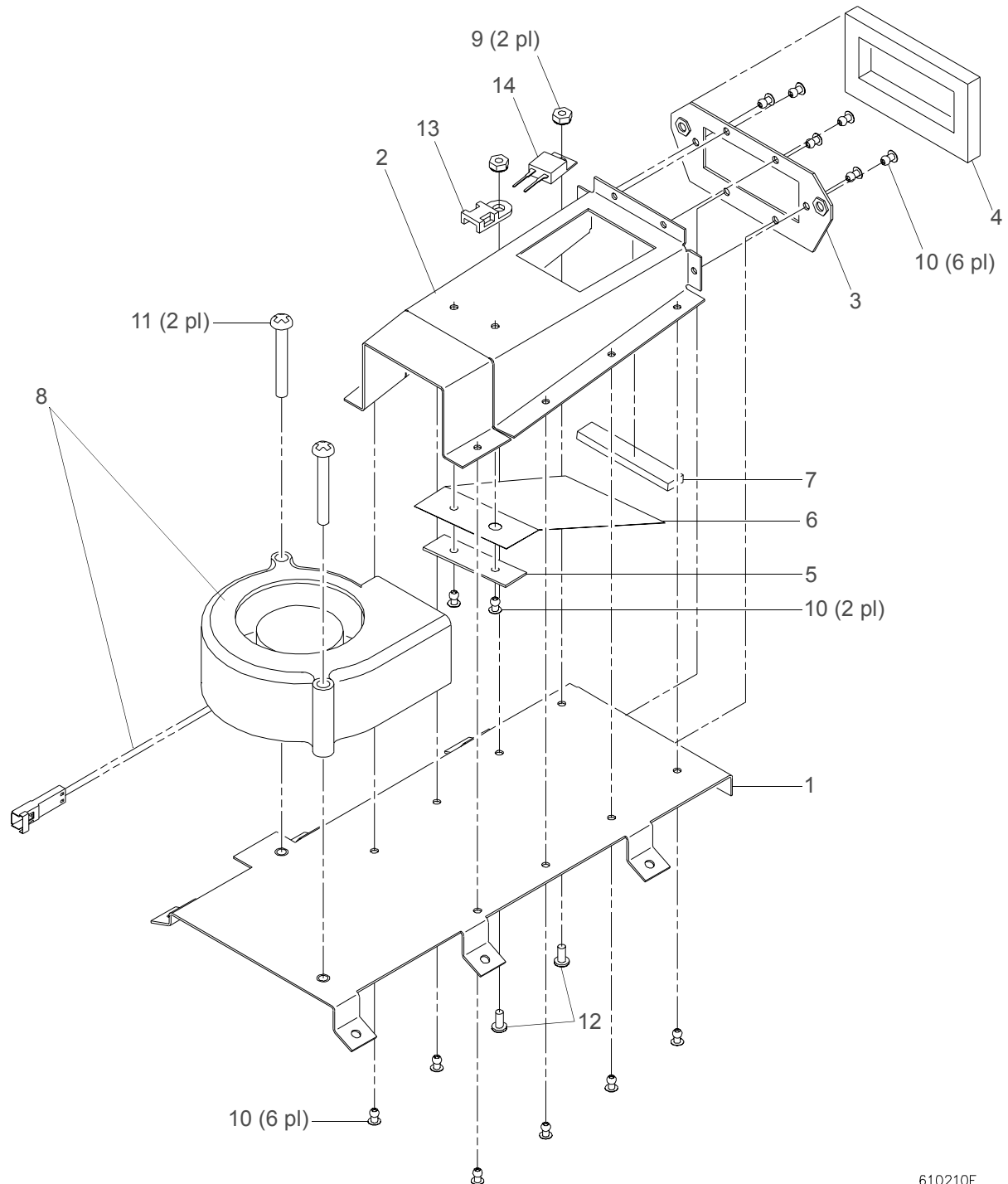
Figure 3-8: Fan Duct Assembly
