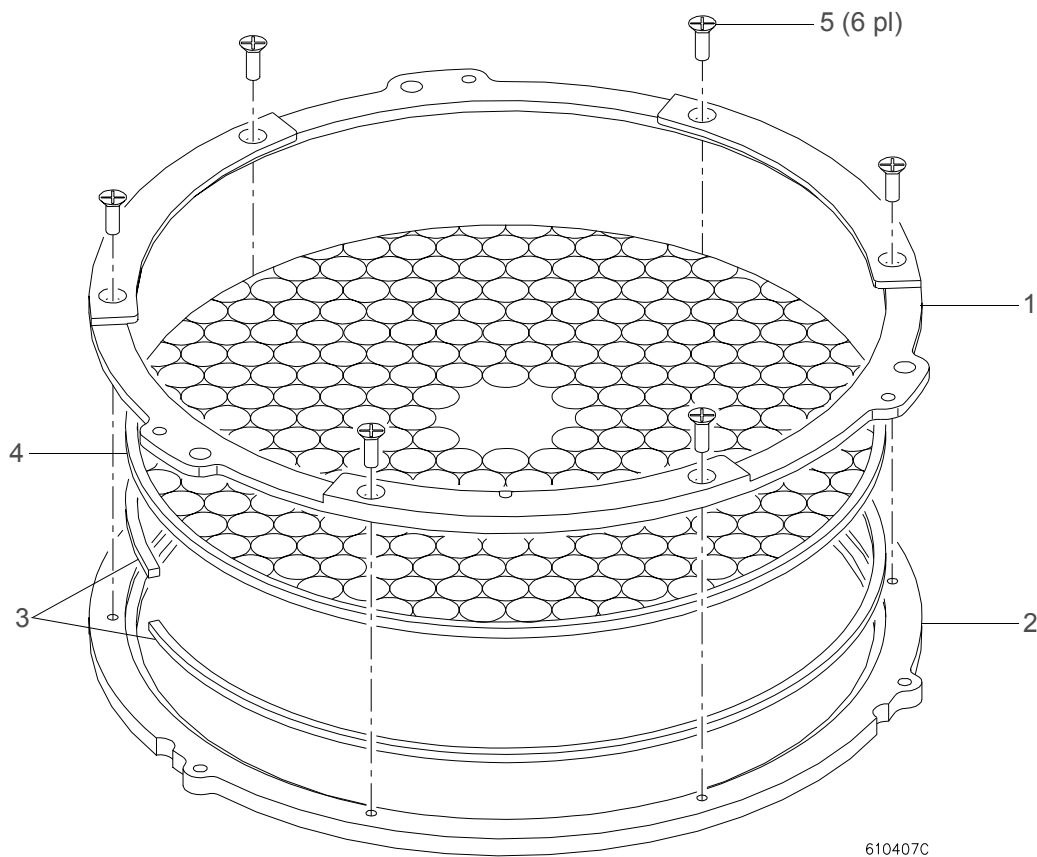
Figure 3-33: Concave Lens Assembly
