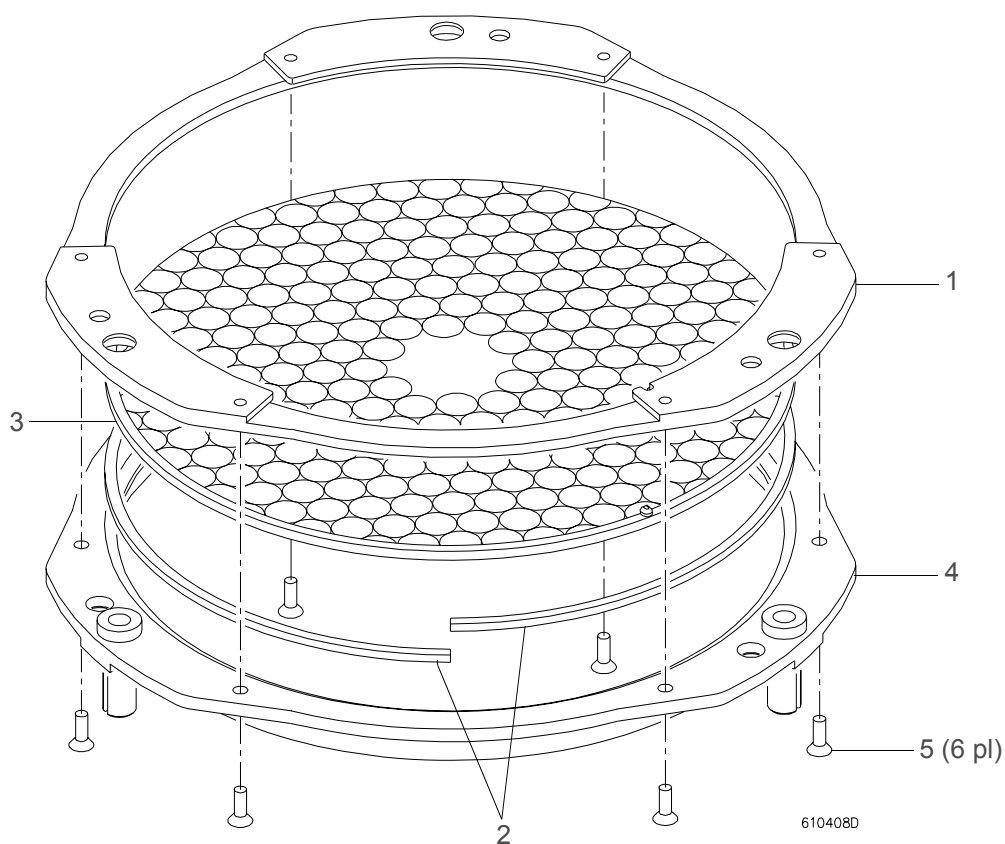
Figure 3-34: Convex Lens Assembly
