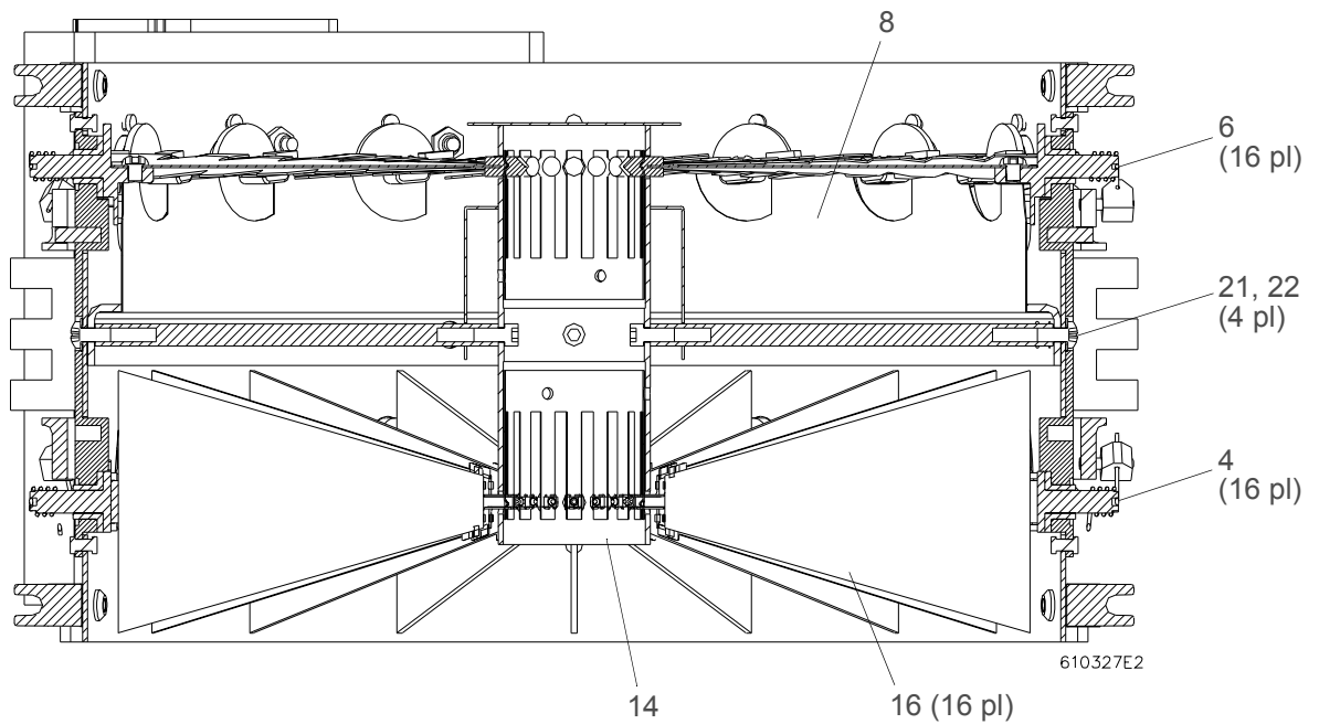
Figure 3-24: Amber/Dimmer Bulkhead Assembly (cutaway view)
