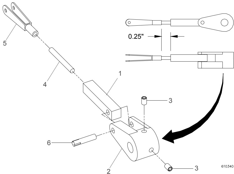
Figure 3-21: Crank Color Strobe Assembly (Old Style)
