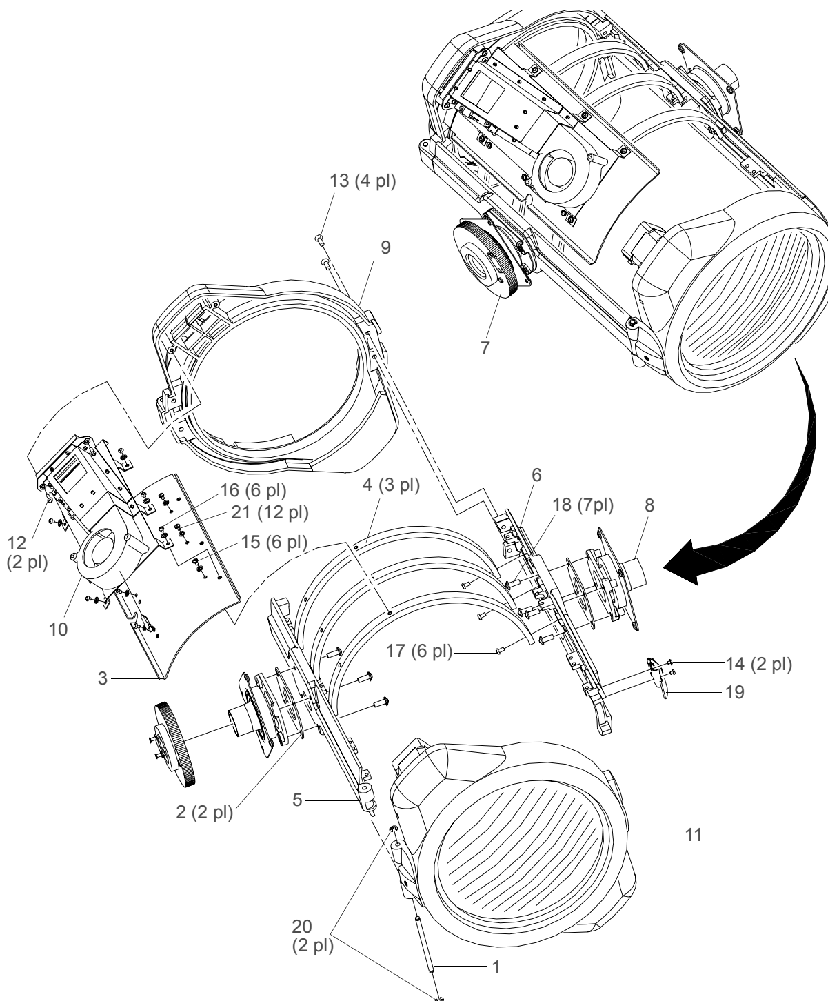
Figure 3-5: Chassis Assembly
