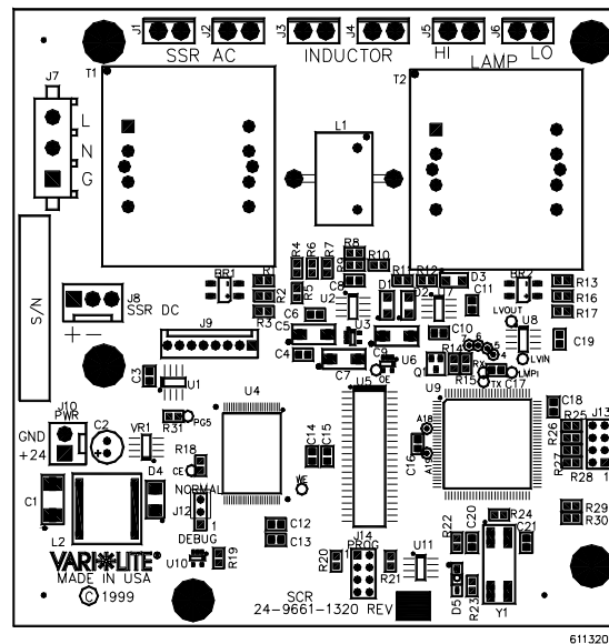
Figure 3-53: 1200W Source Dimmer Control PCB Assembly
