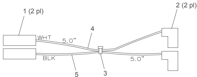
Figure 3-65: AC Input Link Cable Assembly
