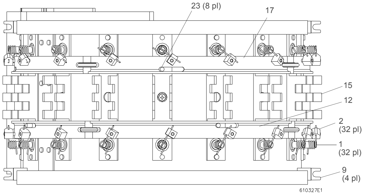
Figure 3-23: Amber/Dimmer Bulkhead Assembly (side view)
