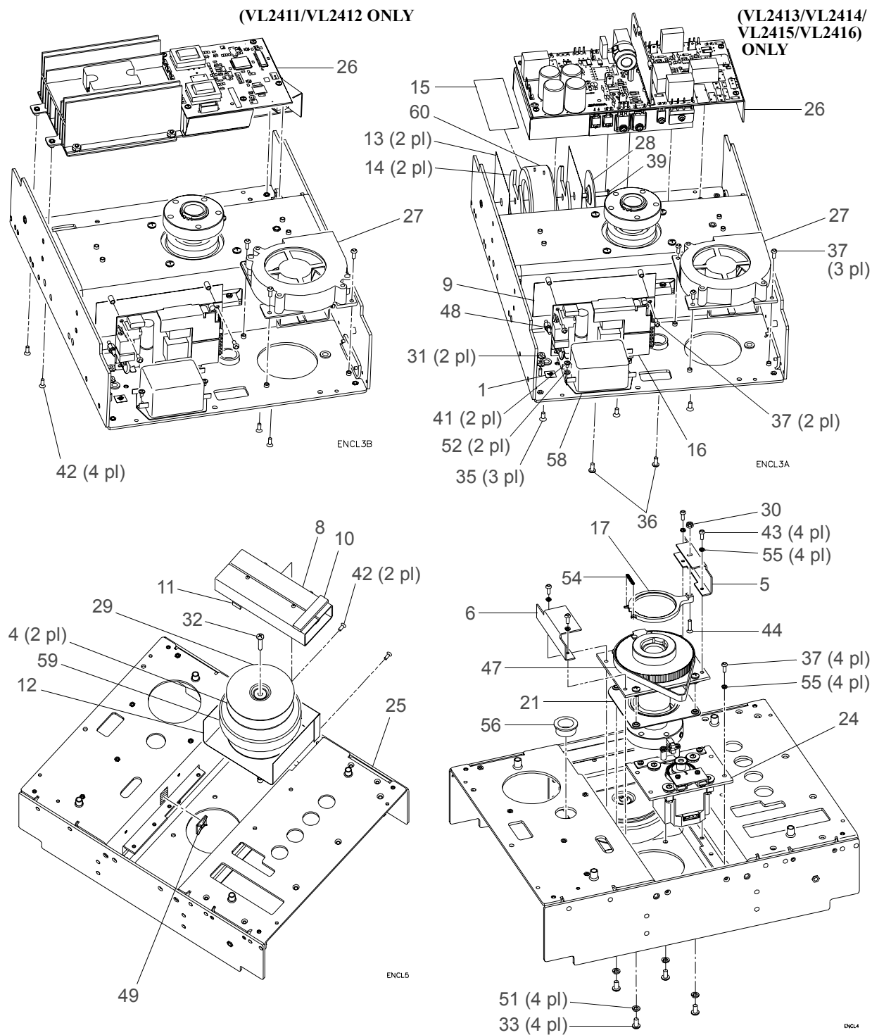
Figure 3-45: Enclosure Assembly (bottom views)
