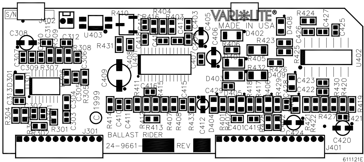
Figure 3-57: 400/625W Ballast Rider Board PCB Assembly
