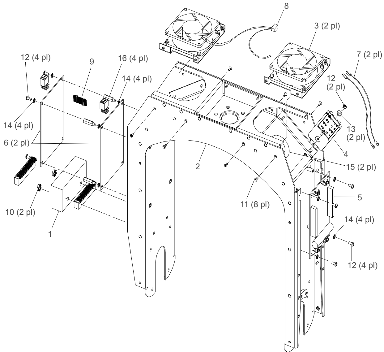
Figure 3-40: Yoke Assembly
