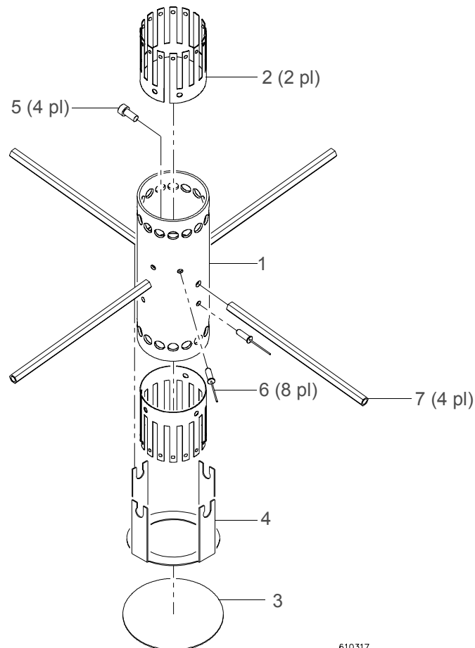
Figure 3-27: Center Hub Assembly
