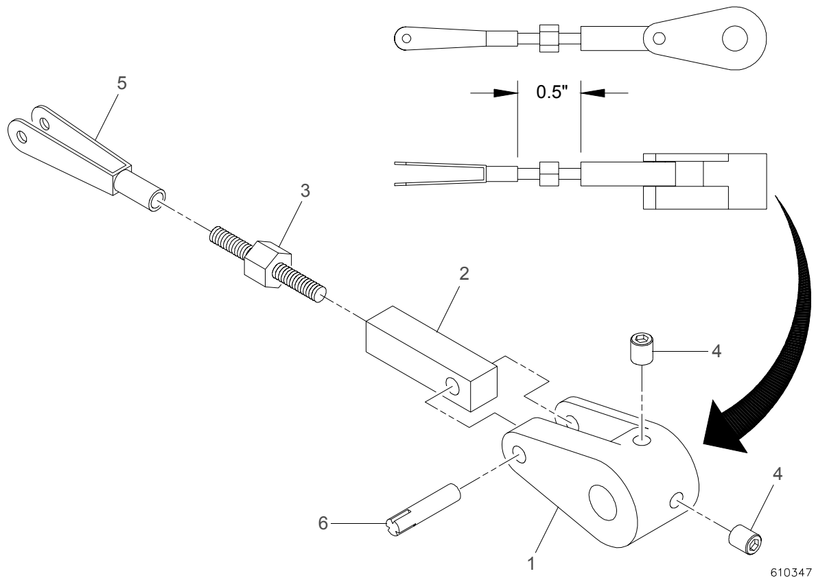
Figure 3-20: Adjustable Crank Color Strobe Assembly
