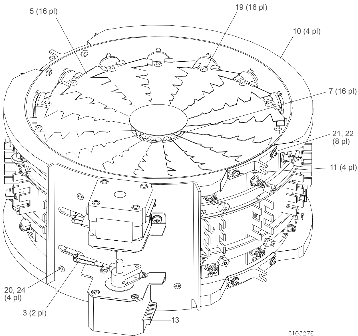
Figure 3-25: Amber/Dimmer Bulkhead Assembly (three-quarters view)
