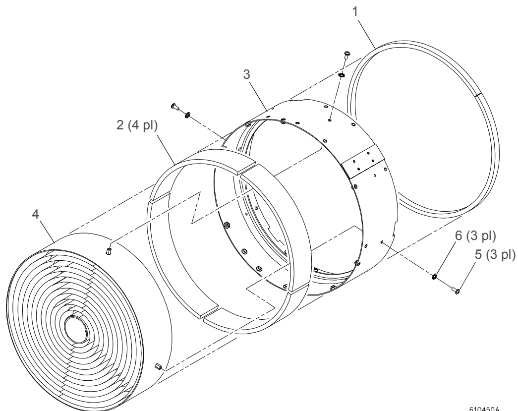
Figure 3-38: Light Baffle Ring Bulkhead Assembly
