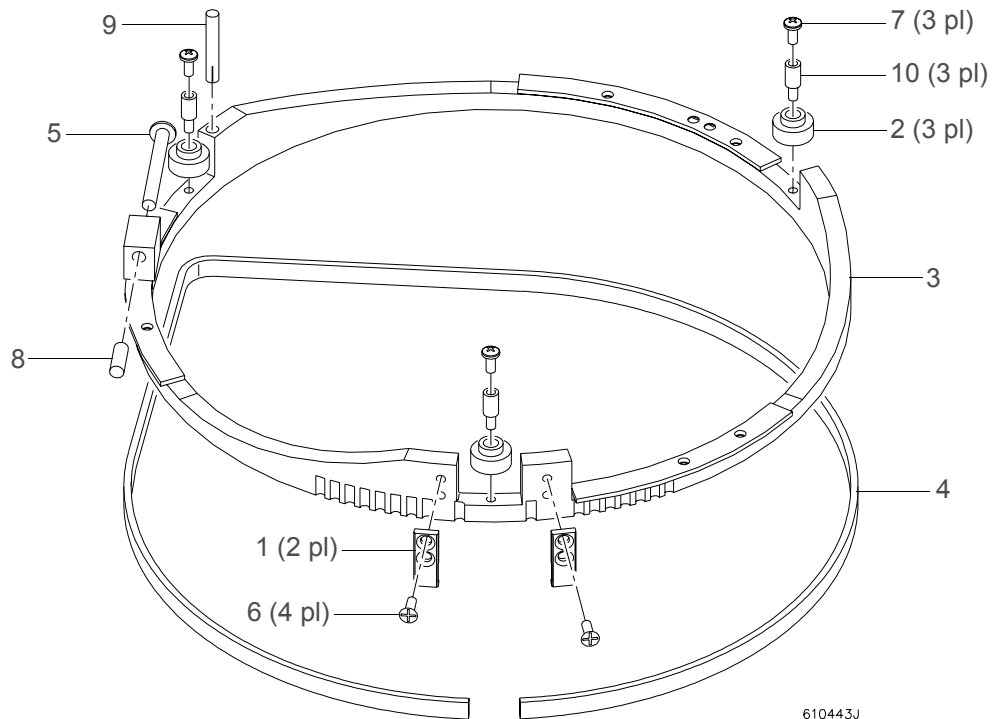
Figure 3-37: Cam Ring Assembly
