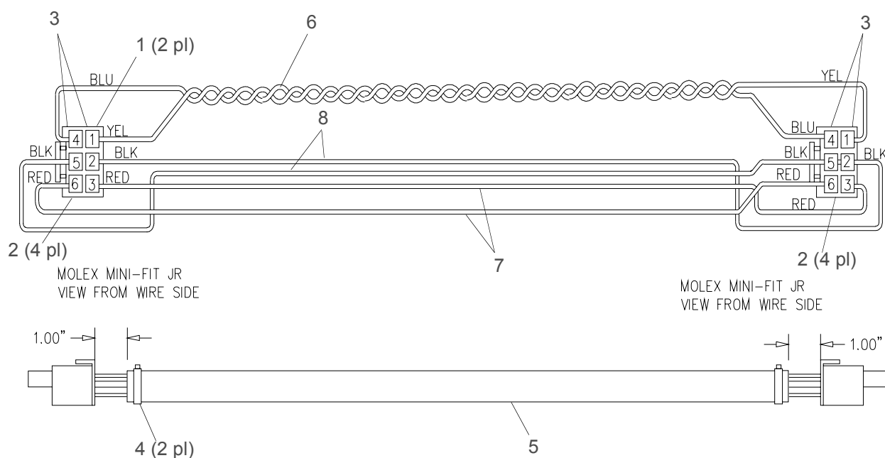
Figure 3-68: Main to Aux/Data & Power Cable Assembly
