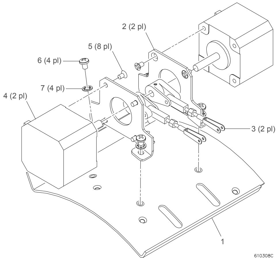
Figure 3-19: Blue/Magenta Motor Assembly
