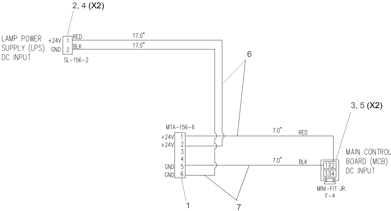
Figure 3-82: DC Output XPiQ Cable Assembly
