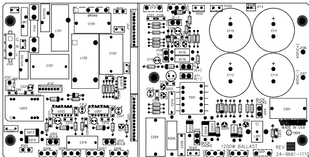
Figure 3-60: 1200W Ballast PCB Assembly
