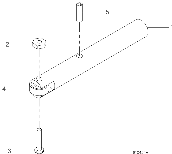
Figure 3-35: Cam Follower Shaft Assembly
