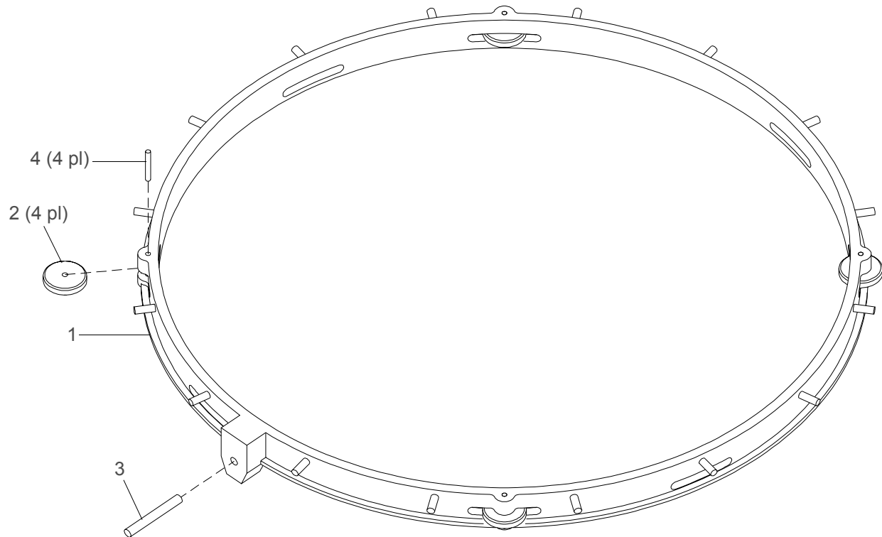
Figure 3-18: Drive Ring Assembly
