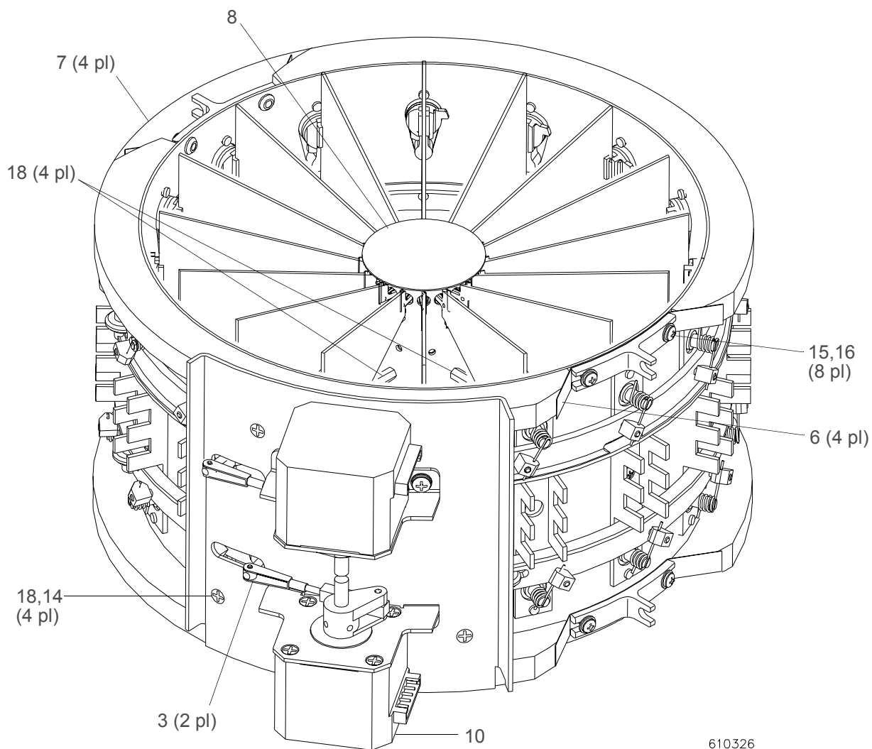
Figure 3-16: Blue/Magenta Bulkhead Assembly (three-quarter view)
