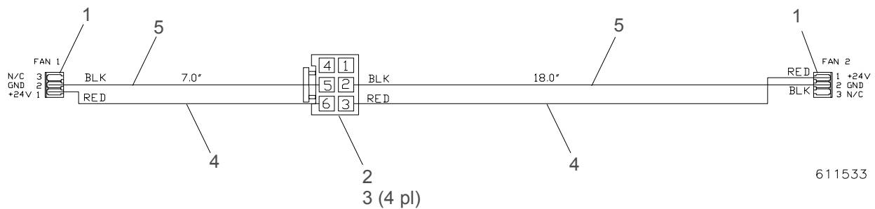
Figure 3-81: Yoke Fan Power Cable Assembly
