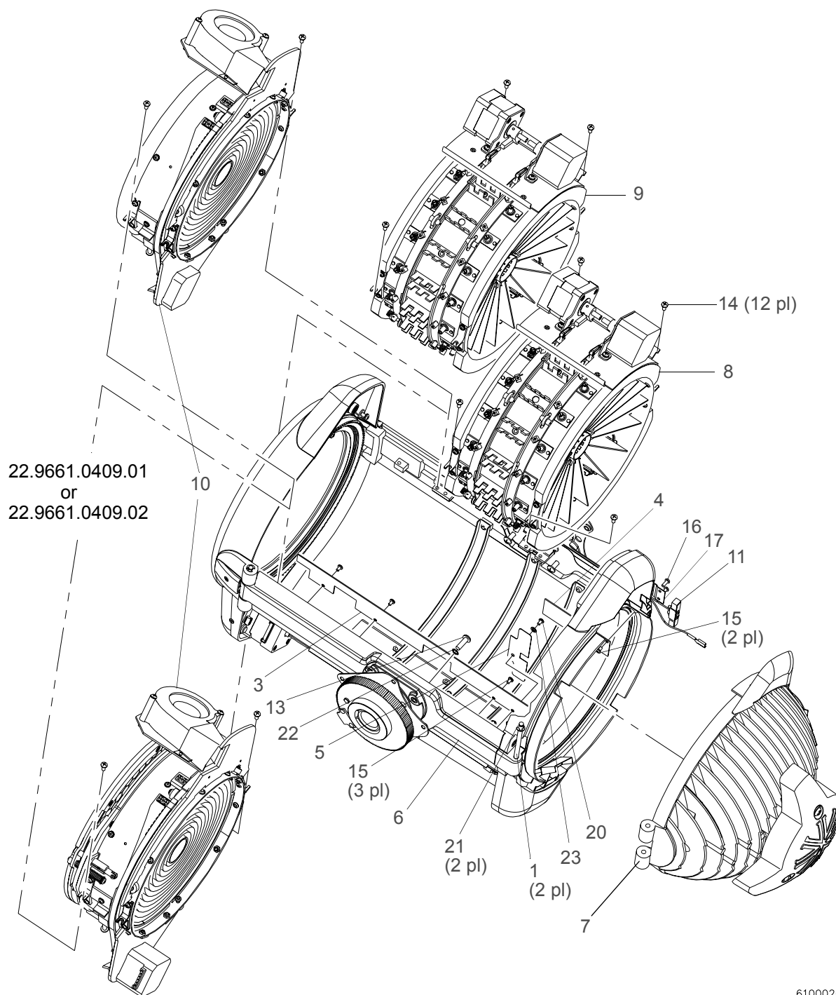
Figure 3-4: Head Assembly
