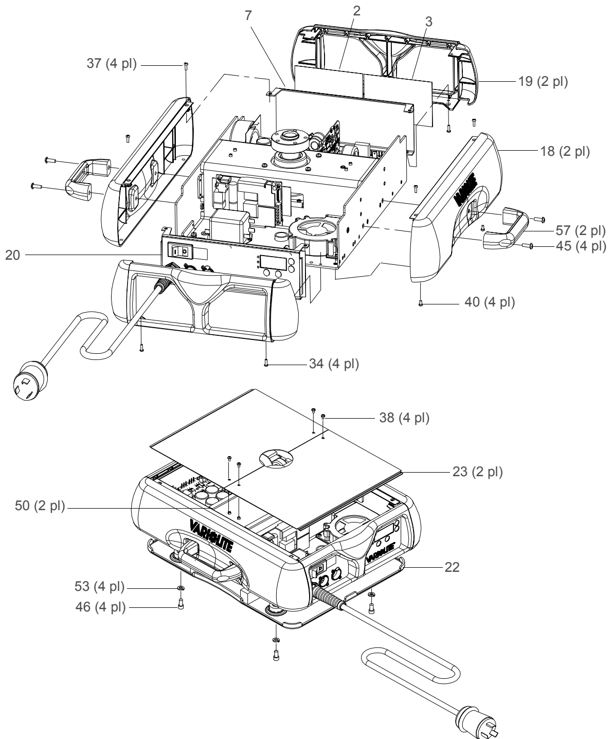
Figure 3-46: Enclosure Assembly (top views)
