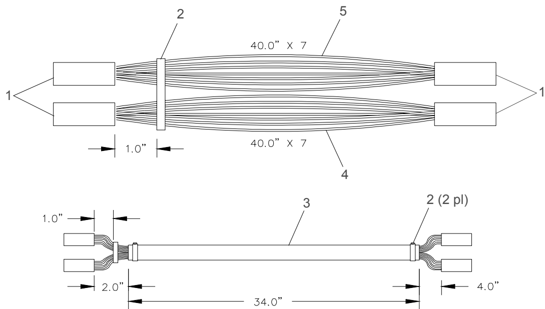
Figure 3-75: Lamp Supply To Relay -2400 Cable Assembly
