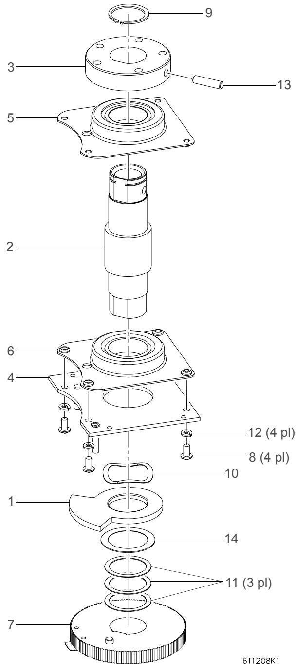
Figure 3-50: Pan Tube Assembly
