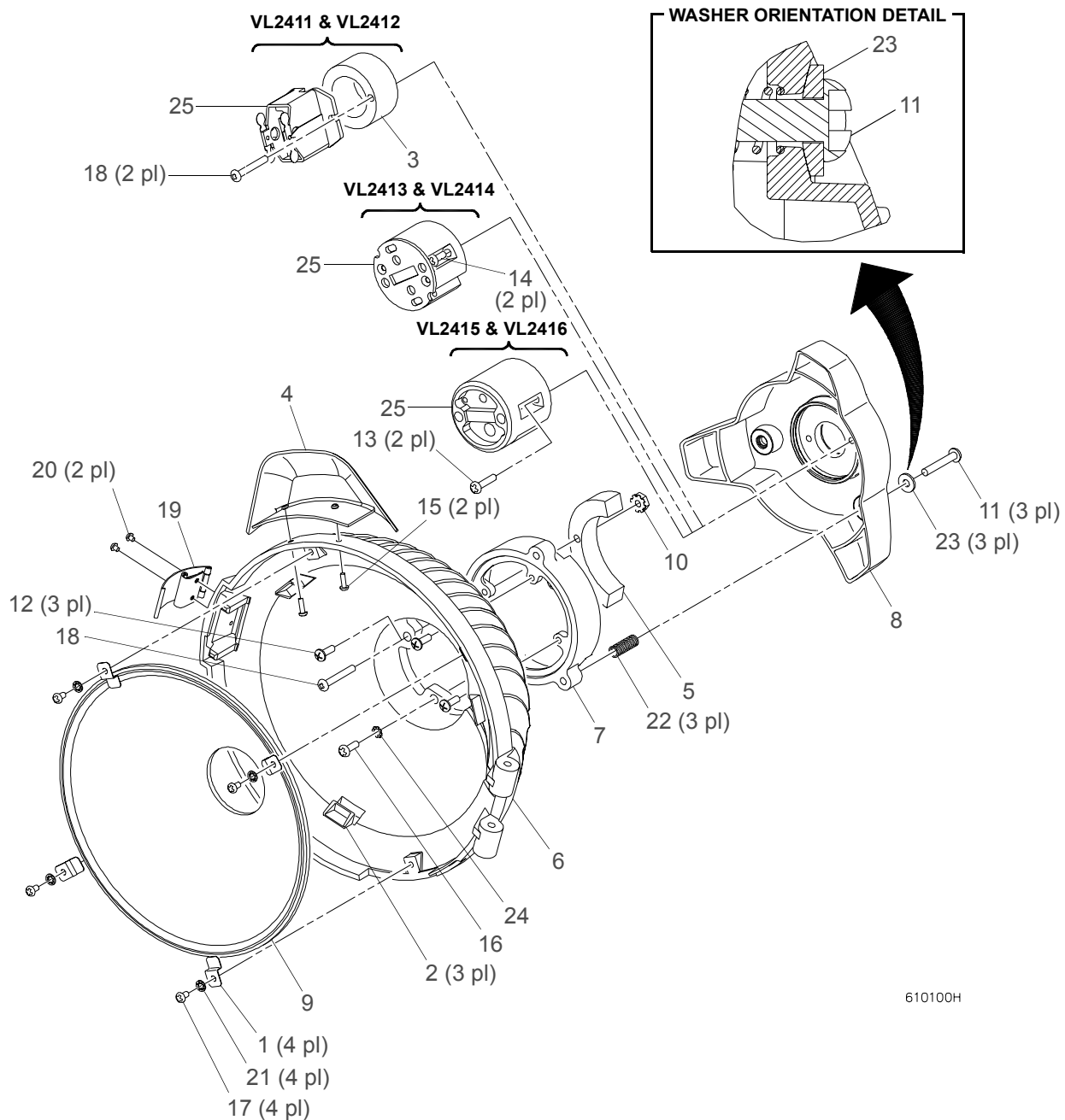
Figure 3-13: Heatsink Assembly
