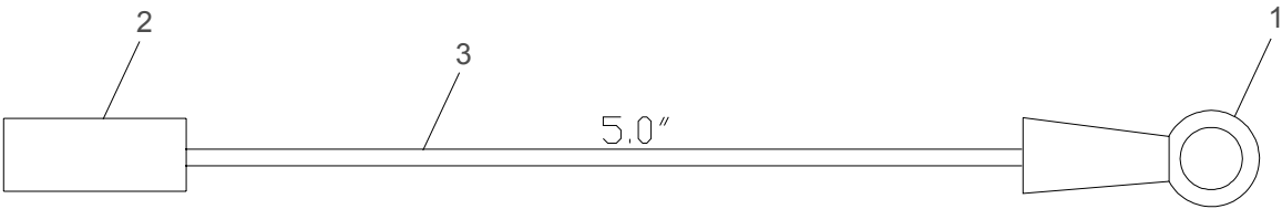
Figure 3-76: Ignitor to Relay Cable Assembly
