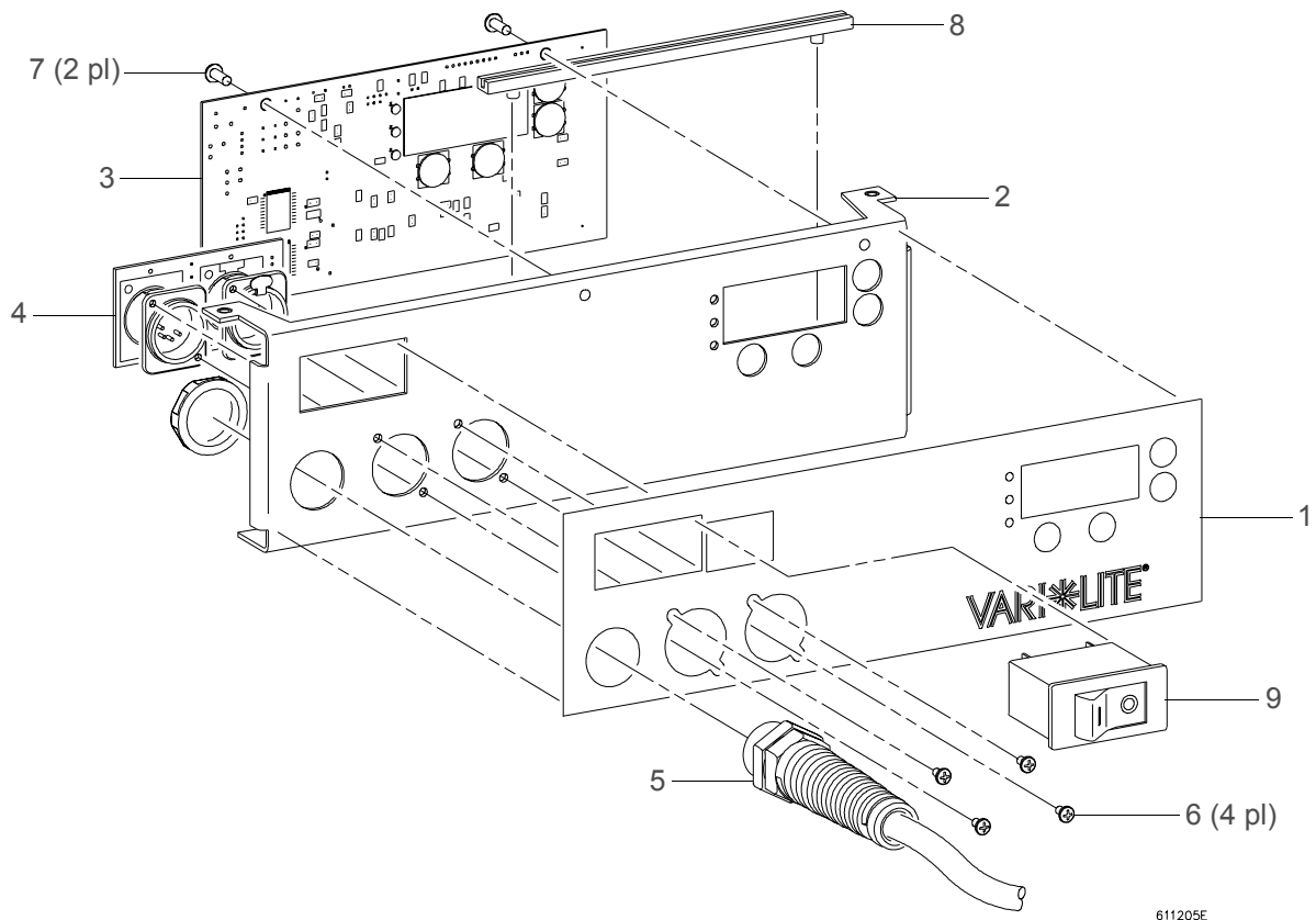
Figure 3-47: Connector Panel Assembly
