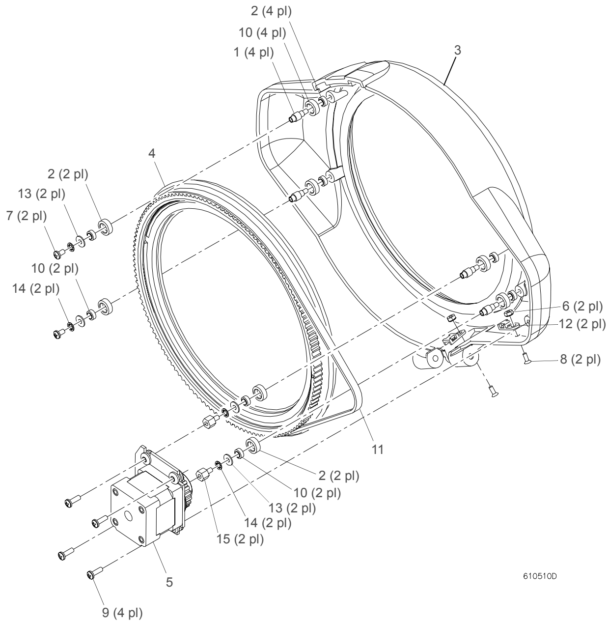
Figure 3-10: Front Ring Assembly
