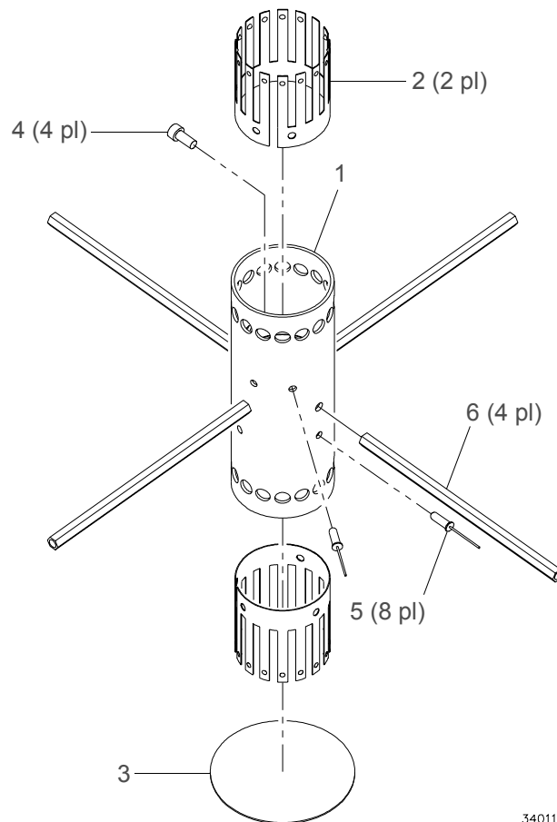
Figure 3-17: Center Hub Assembly
