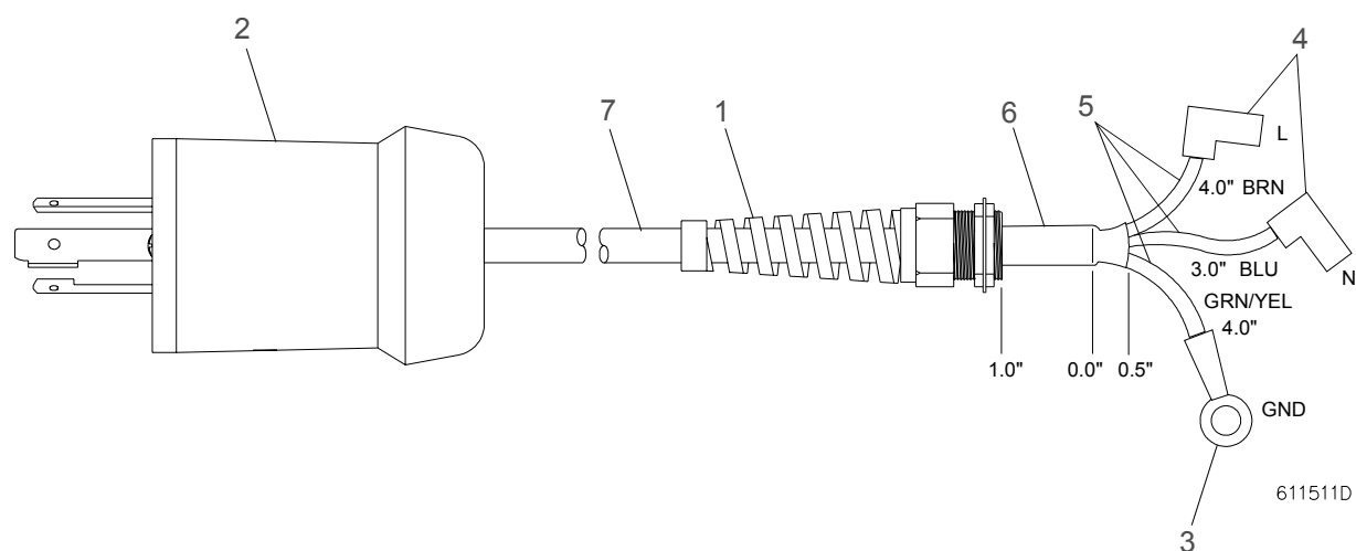
Figure 3-64: AC Input Pigtail (Euro) Cable Assembly
