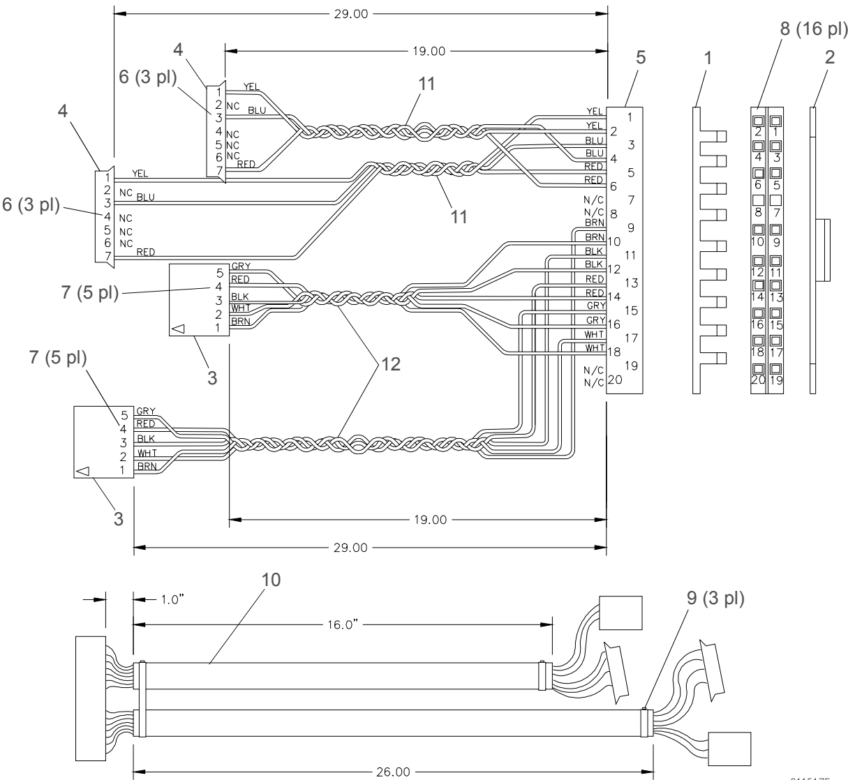
Figure 3-69: Pan/Tilt Control - 2400 Cable Assembly
