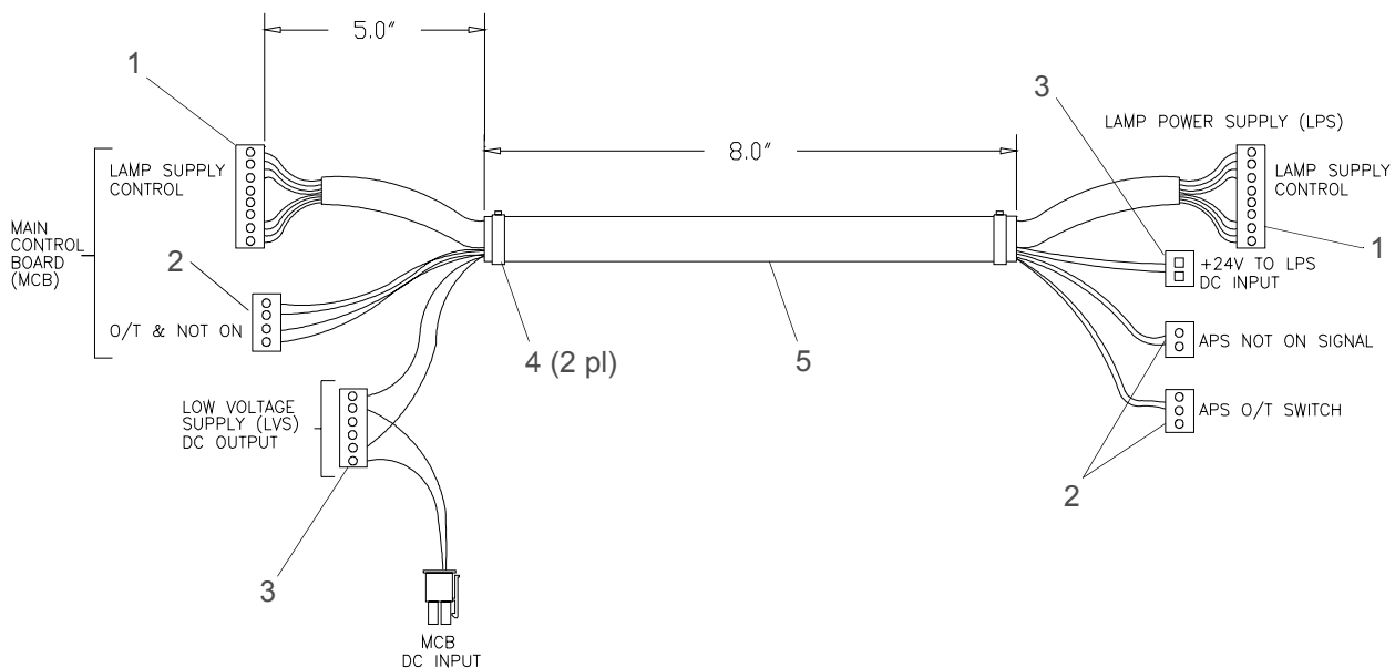
Figure 3-83: Lamp Supply Harness - 2400 Cable Assembly
