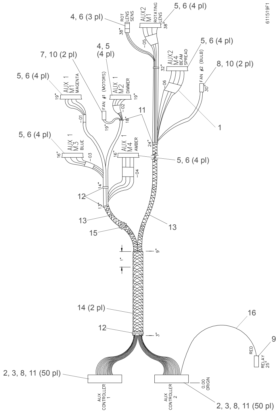
Figure 3-71: Motor Harness Cable Assembly
