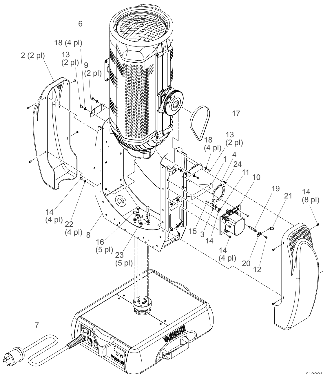
Figure 3-2: Top Assembly
