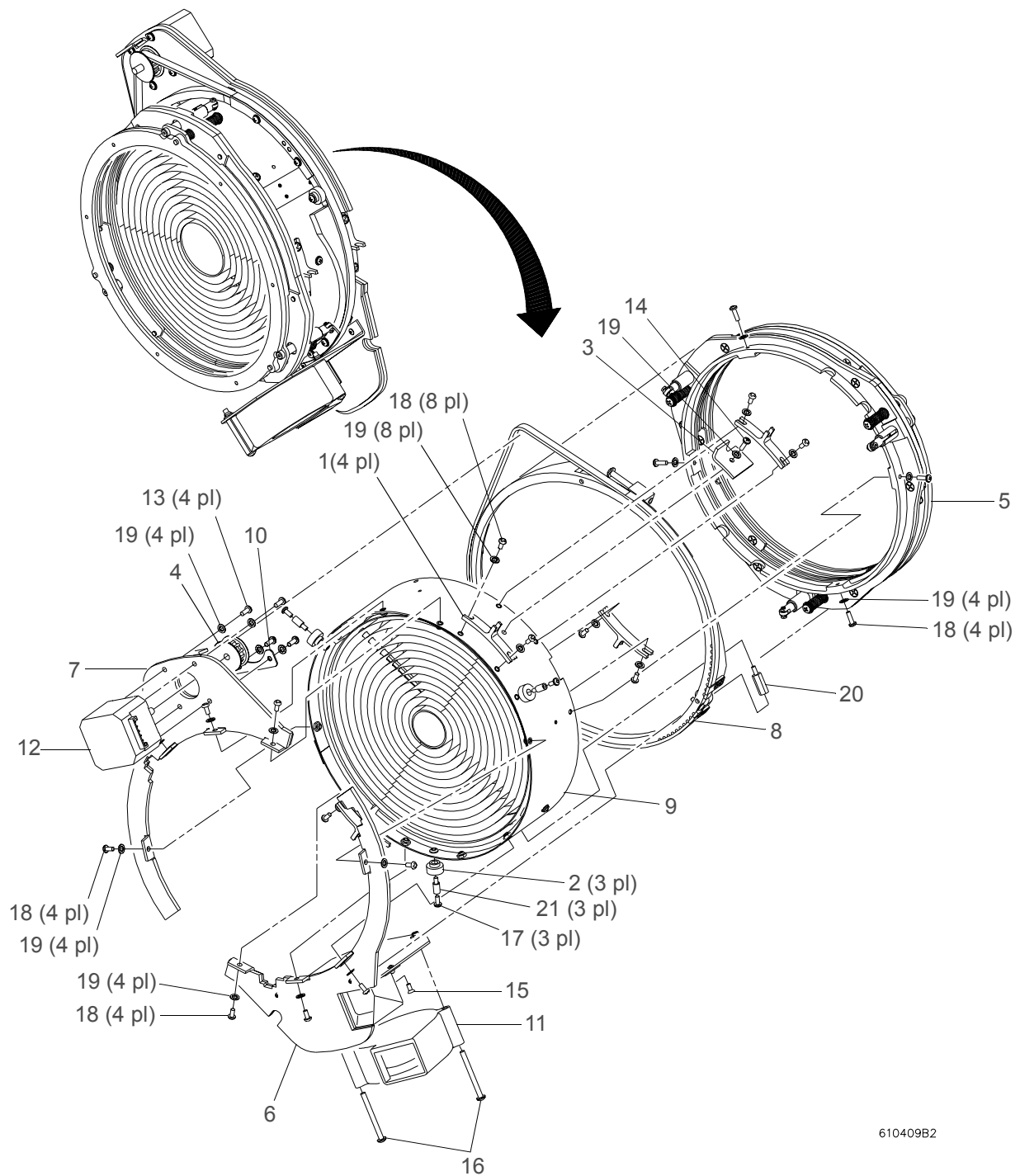
Figure 3-31: Baffle/Beam Spreader Assembly VL2412/VL2414/VL2416
