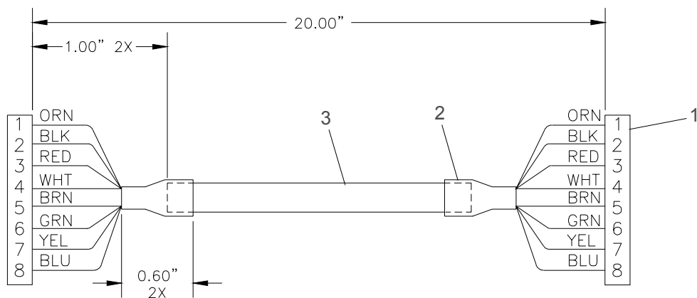
Figure 3-70: Lamp Supply Control Cable Assembly
