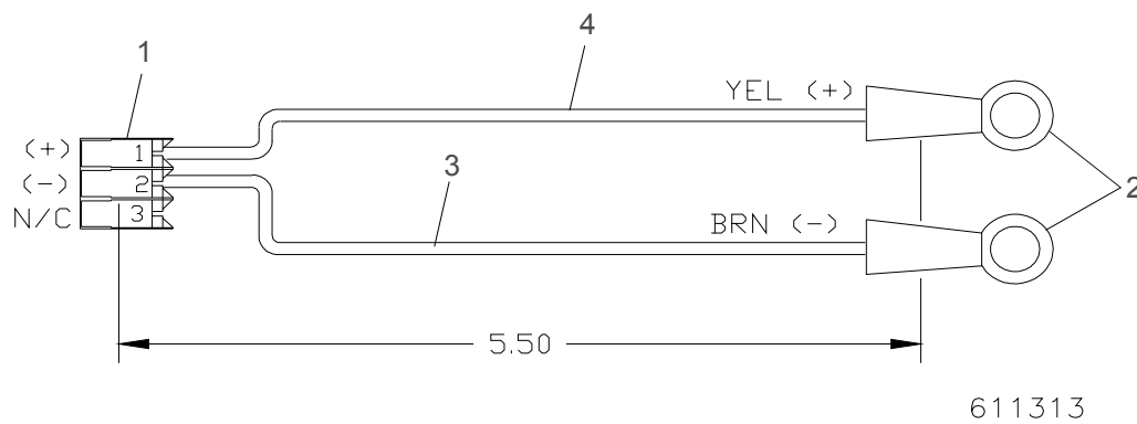
Figure 3-63: SSR DC Cable Assembly
