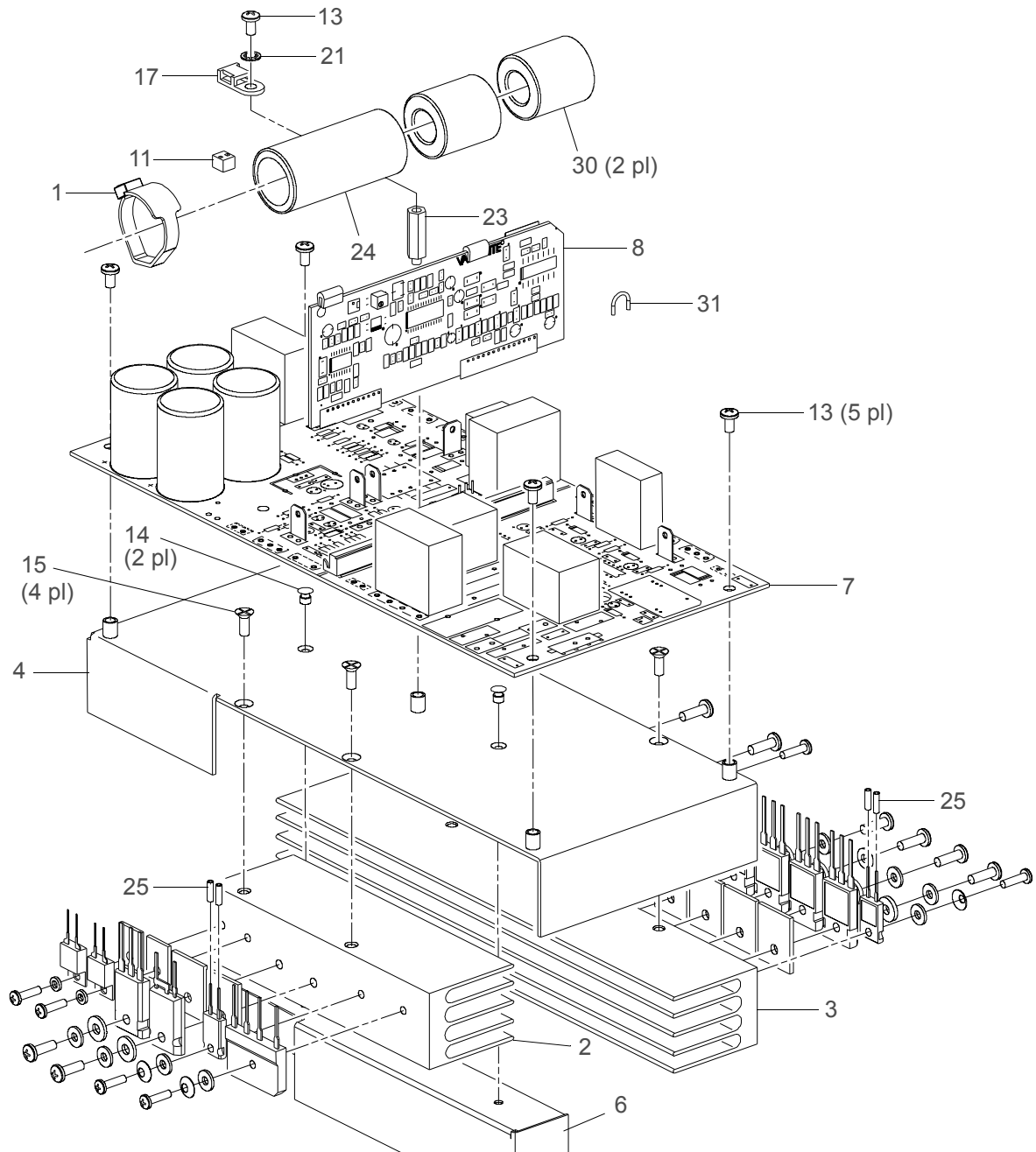
Figure 3-54: 625W Arc Ballast Module Assembly
