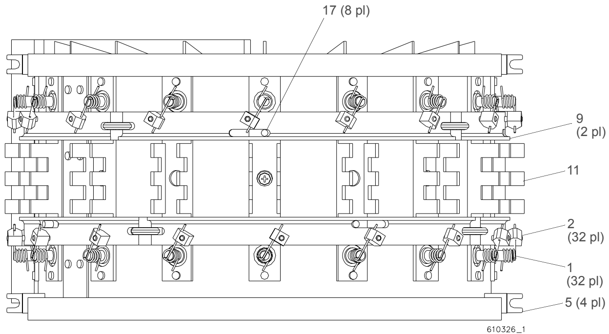
Figure 3-14: Blue/Magenta Bulkhead Assembly (side view)
