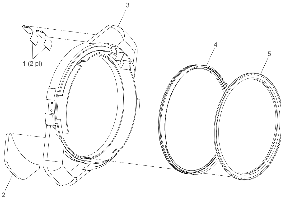
Figure 3-6: Cooling Bulkhead Assembly VL2411/VL2412
