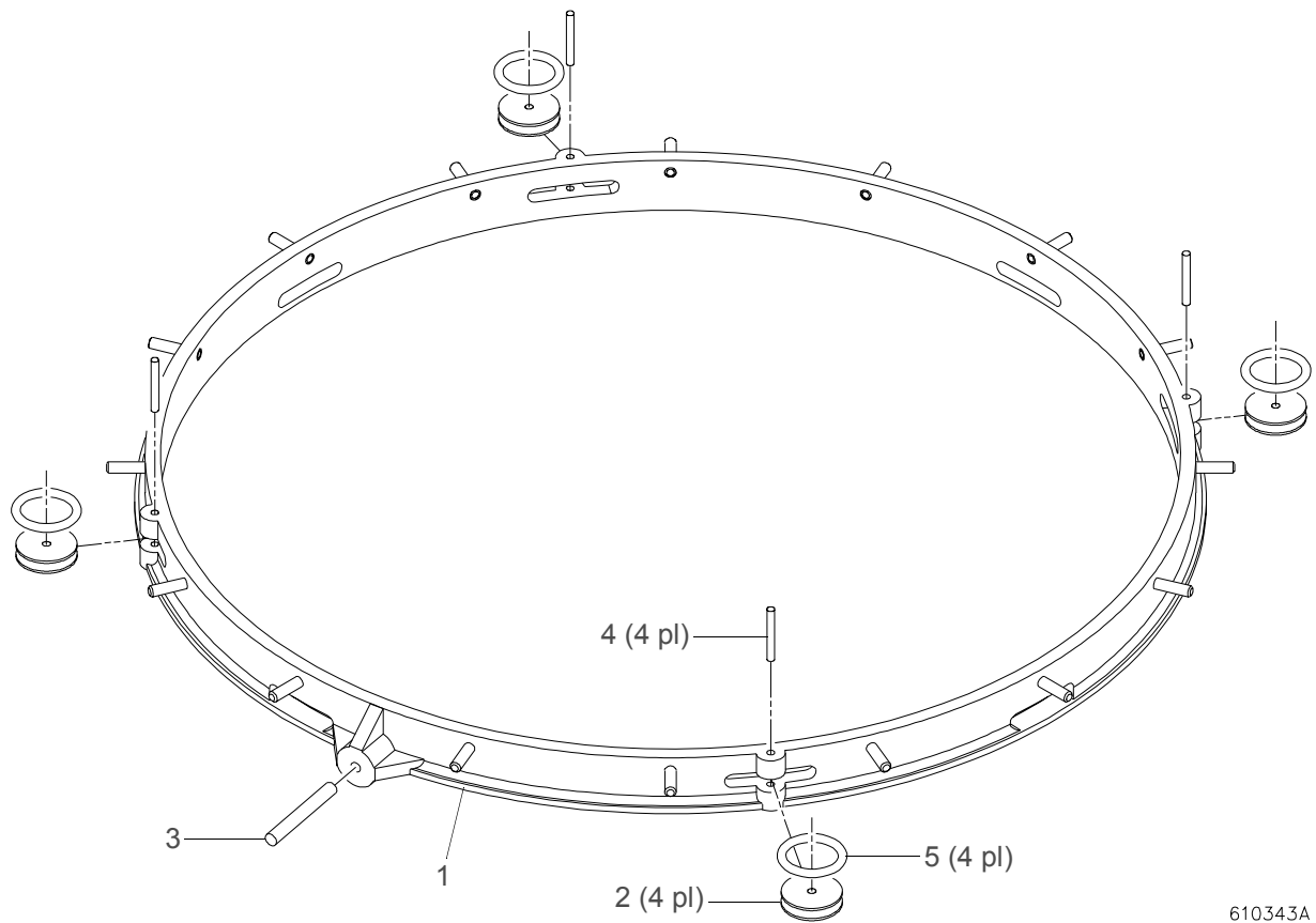
Figure 3-28: Strobe Drive Ring Assembly
