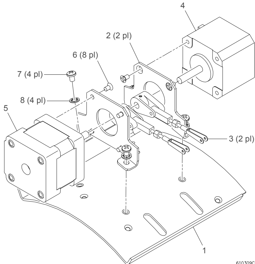
Figure 3-26: Amber/Dimmer Motor Assembly
