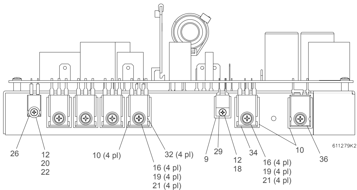
Figure 3-55: 625W Arc Ballast Module Assembly (side views)
