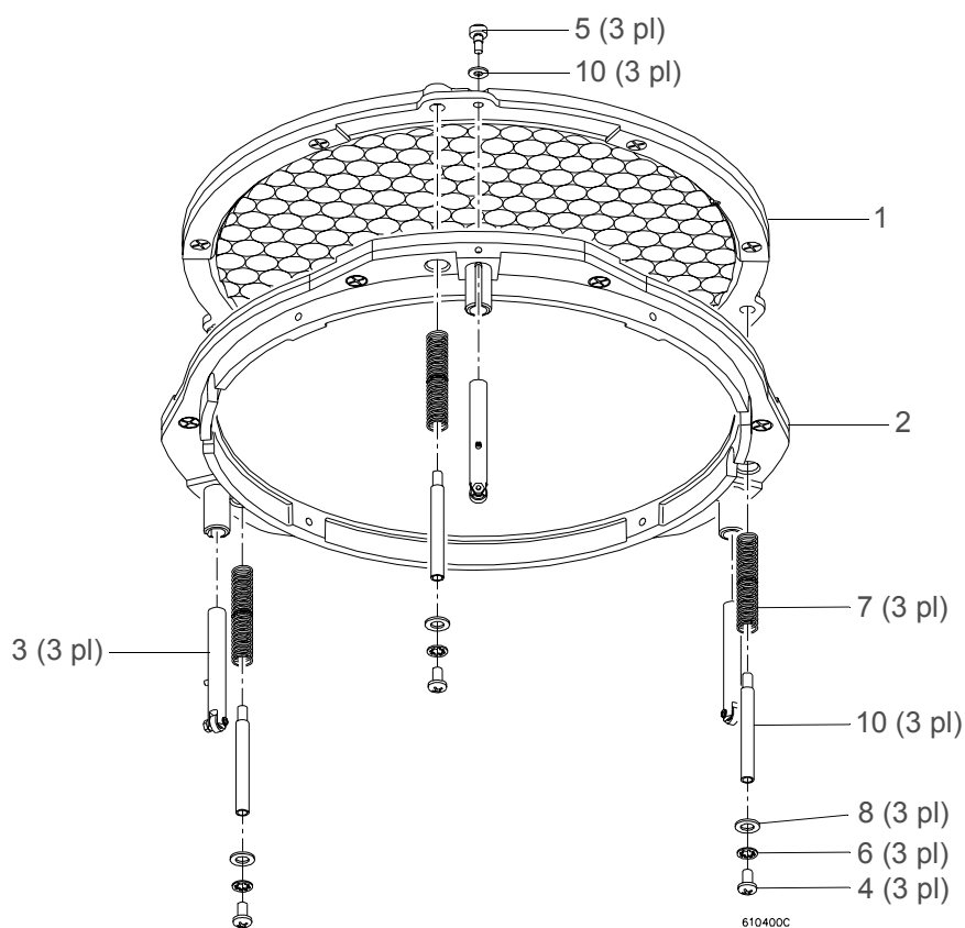
Figure 3-32: Beam Spreader Assembly
