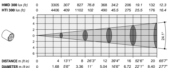
Optional multi-element lens 1:2.8 / 120 mm (24.1°)
