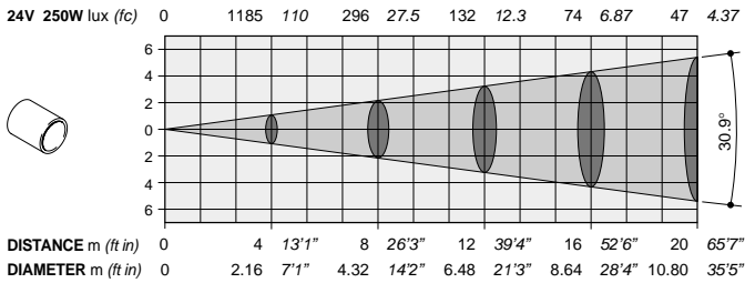
Standard lens 1:2.4 / 100 mm (30.9°)
