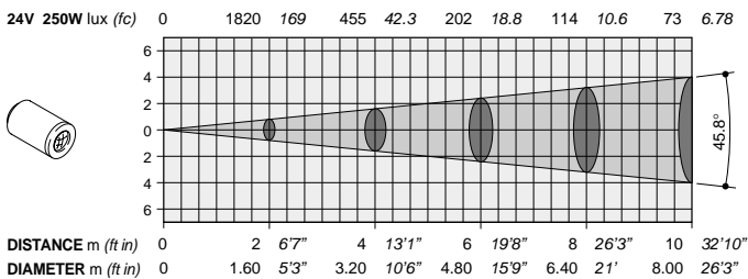
Optional multi-element lens 1:2.8 / 60mm (45.8°)
