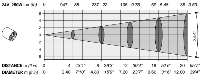
Optional multi-element lens 1:2.8 / 85 mm (34.4°)
