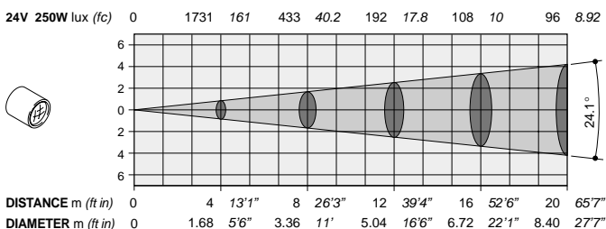
Optional multi-element lens 1:2.8 / 120 mm (24.1°)
