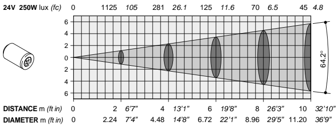
Optional multi-element lens 1:2.8 / 45mm (64.2°)
