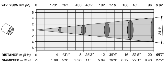
Optional multi-element lens 1:2.8 / 120 mm (24.1°)
