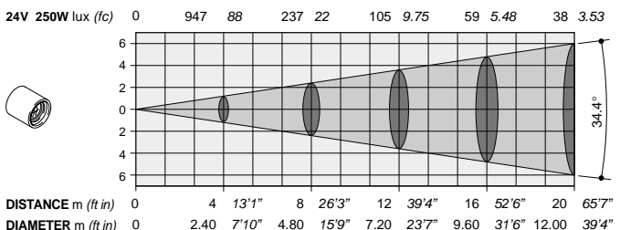
Optional multi-element lens 1:2.8 / 85 mm (34.4°)
