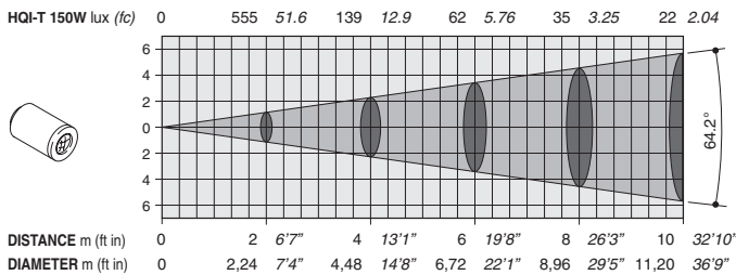
Optional multi-element lens 1:2.8 / 45mm (64.2°)
