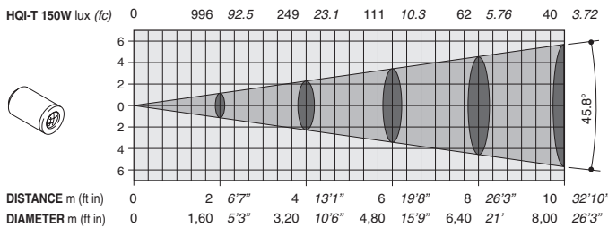
Optional multi-element lens 1:2.8 / 60 mm (45.8°)
