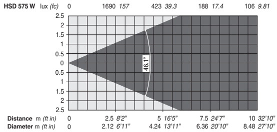
Multi-element lens 1 : 2.8/45 mm (46°)
