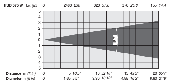
Multi-element lens 1 : 2.8/120 mm (18.7°)
