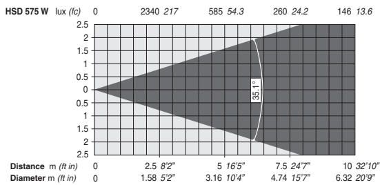
Multi-element lens 1 : 2.8/60 mm (35.1°)
