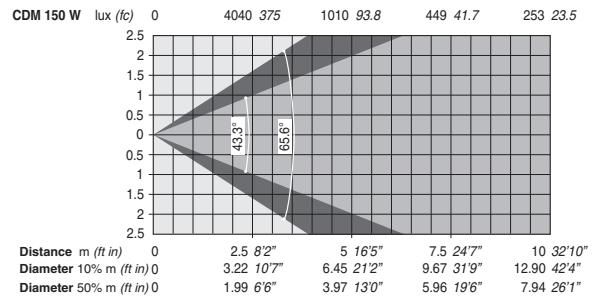
With optional ovalizer filter (X-axis) (65.6° 10% - 43.3° 50%)
