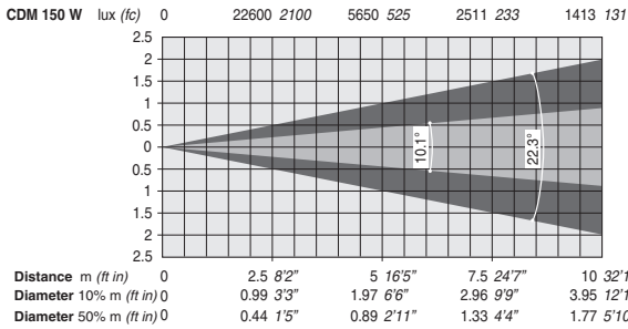
Standard filter only (22.3° 10% - 10.1° 50%)
